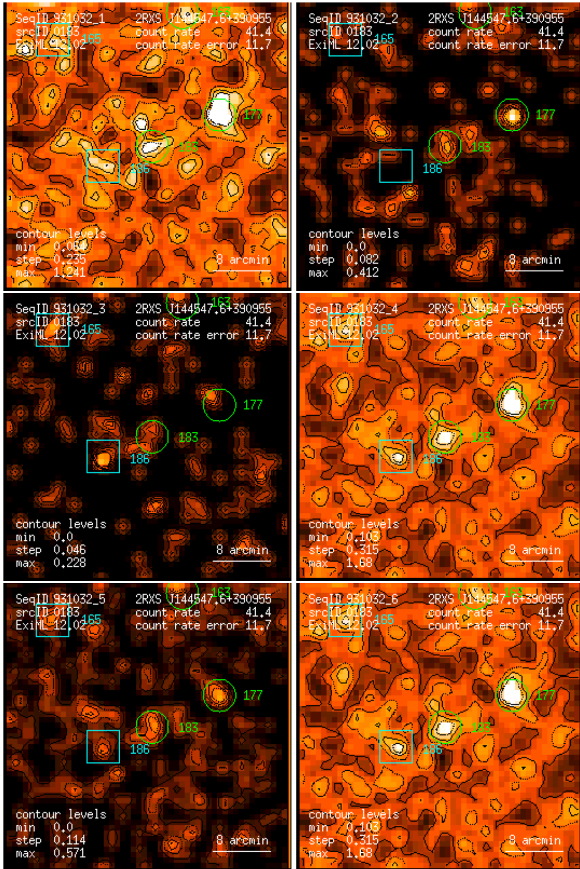
Figure 183: RASS 931032: detection 0183: band rate images, Gaussian filter: (1) PSPC channels 11 – 41, (2) 52 – 90, (3) 91 – 201, (4) 11 – 235, (5) 52 – 201, (6) 11 – 201. Broad band rates in counts/ks. Band rate contour levels in counts/ks/arcmin 2 .
