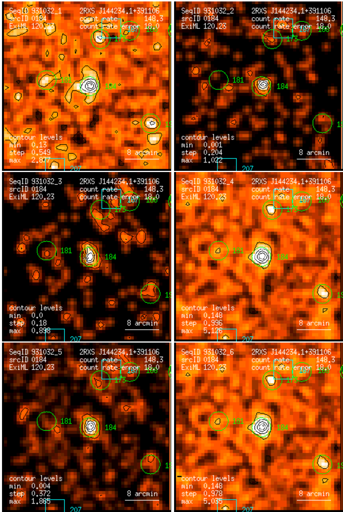
Figure 184: RASS 931032: detection 0184: band rate images, Gaussian filter: (1) PSPC channels 11 – 41, (2) 52 – 90, (3) 91 – 201, (4) 11 – 235, (5) 52 – 201, (6) 11 – 201. Broad band rates in counts/ks. Band rate contour levels in counts/ks/arcmin 2 .
