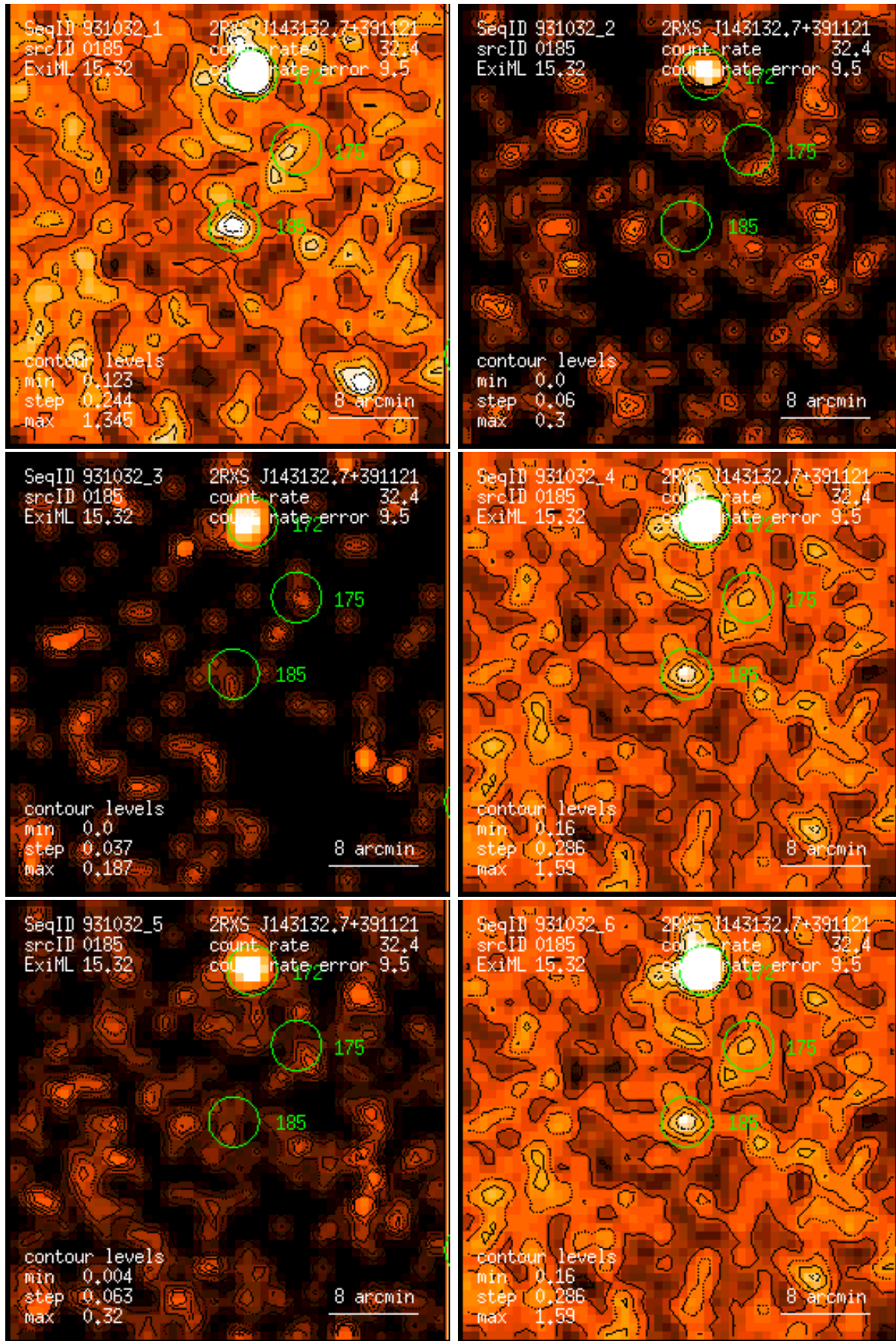
Figure 185: RASS 931032: detection 0185: band rate images, Gaussian filter: (1) PSPC channels 11 – 41, (2) 52 – 90, (3) 91 – 201, (4) 11 – 235, (5) 52 – 201, (6) 11 – 201. Broad band rates in counts/ks. Band rate contour levels in counts/ks/arcmin 2 .
