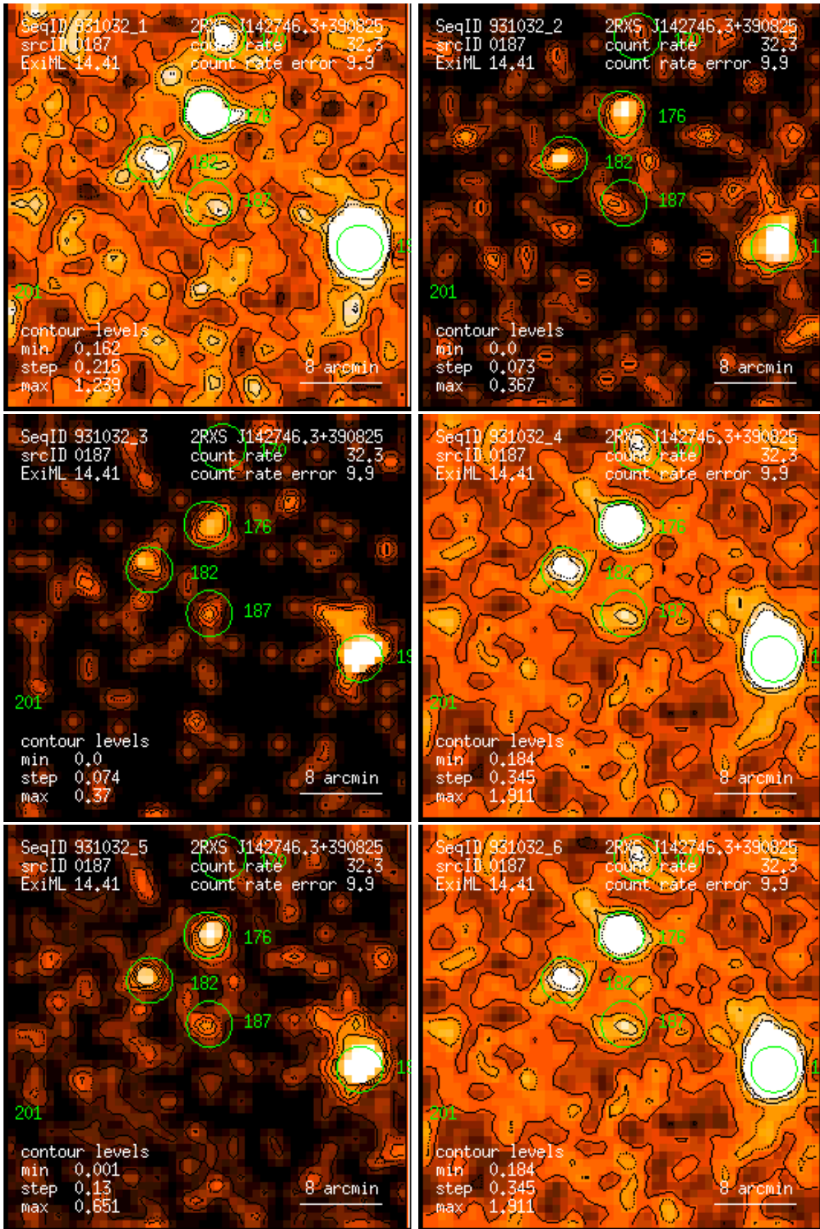
Figure 187: RASS 931032: detection 0187: band rate images, Gaussian filter: (1) PSPC channels 11 – 41, (2) 52 – 90, (3) 91 – 201, (4) 11 – 235, (5) 52 – 201, (6) 11 – 201. Broad band rates in counts/ks. Band rate contour levels in counts/ks/arcmin 2 .
