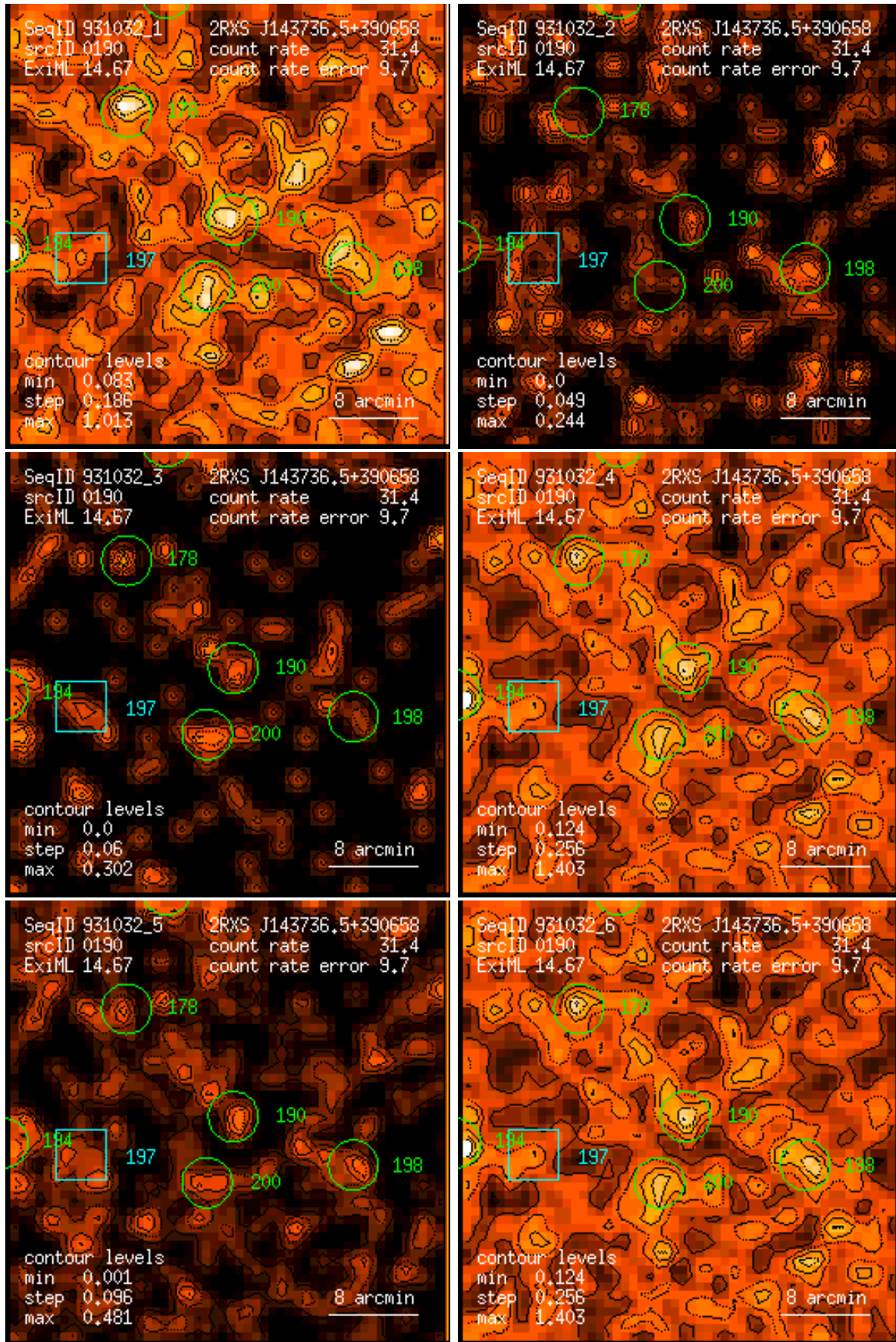
Figure 190: RASS 931032: detection 0190: band rate images, Gaussian filter: (1) PSPC channels 11 – 41, (2) 52 – 90, (3) 91 – 201, (4) 11 – 235, (5) 52 – 201, (6) 11 – 201. Broad band rates in counts/ks. Band rate contour levels in counts/ks/arcmin 2 .
