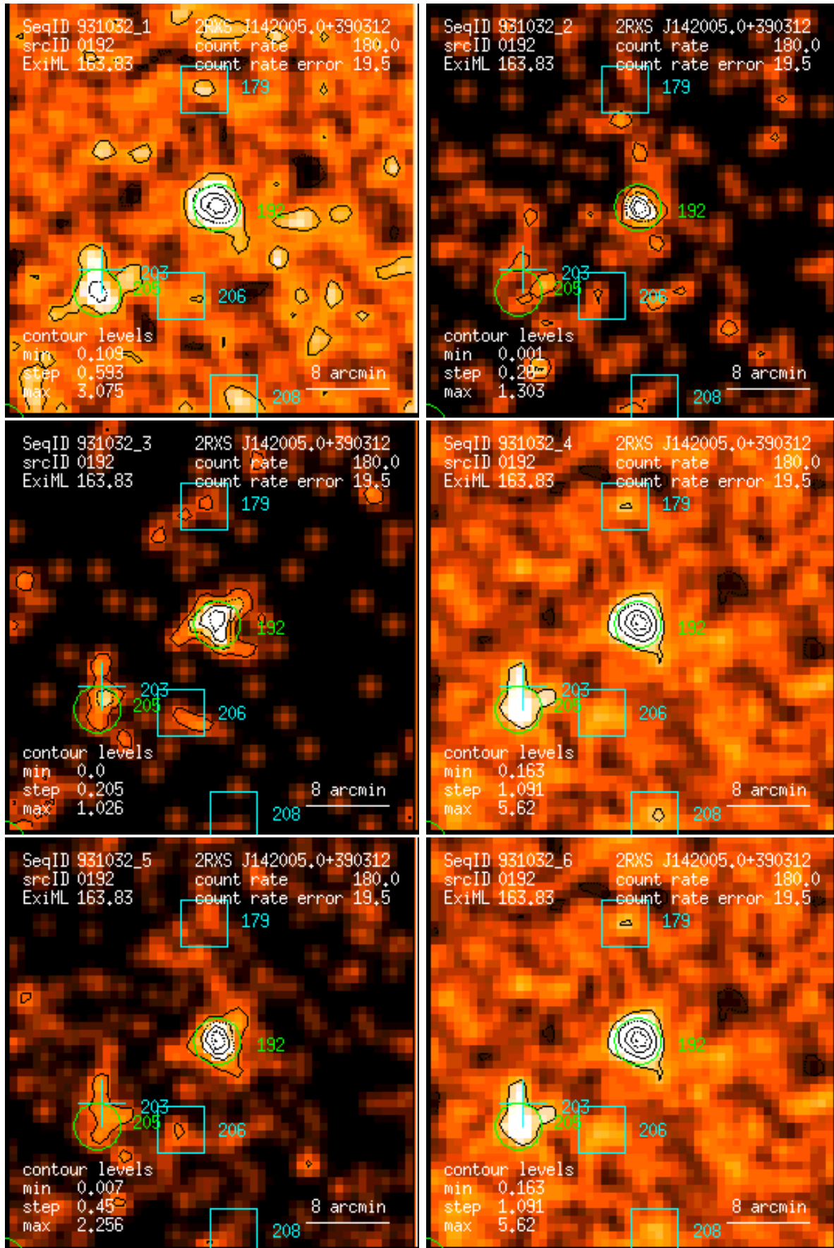
Figure 192: RASS 931032: detection 0192: band rate images, Gaussian filter: (1) PSPC channels 11 – 41, (2) 52 – 90, (3) 91 – 201, (4) 11 – 235, (5) 52 – 201, (6) 11 – 201. Broad band rates in counts/ks. Band rate contour levels in counts/ks/arcmin 2 .
