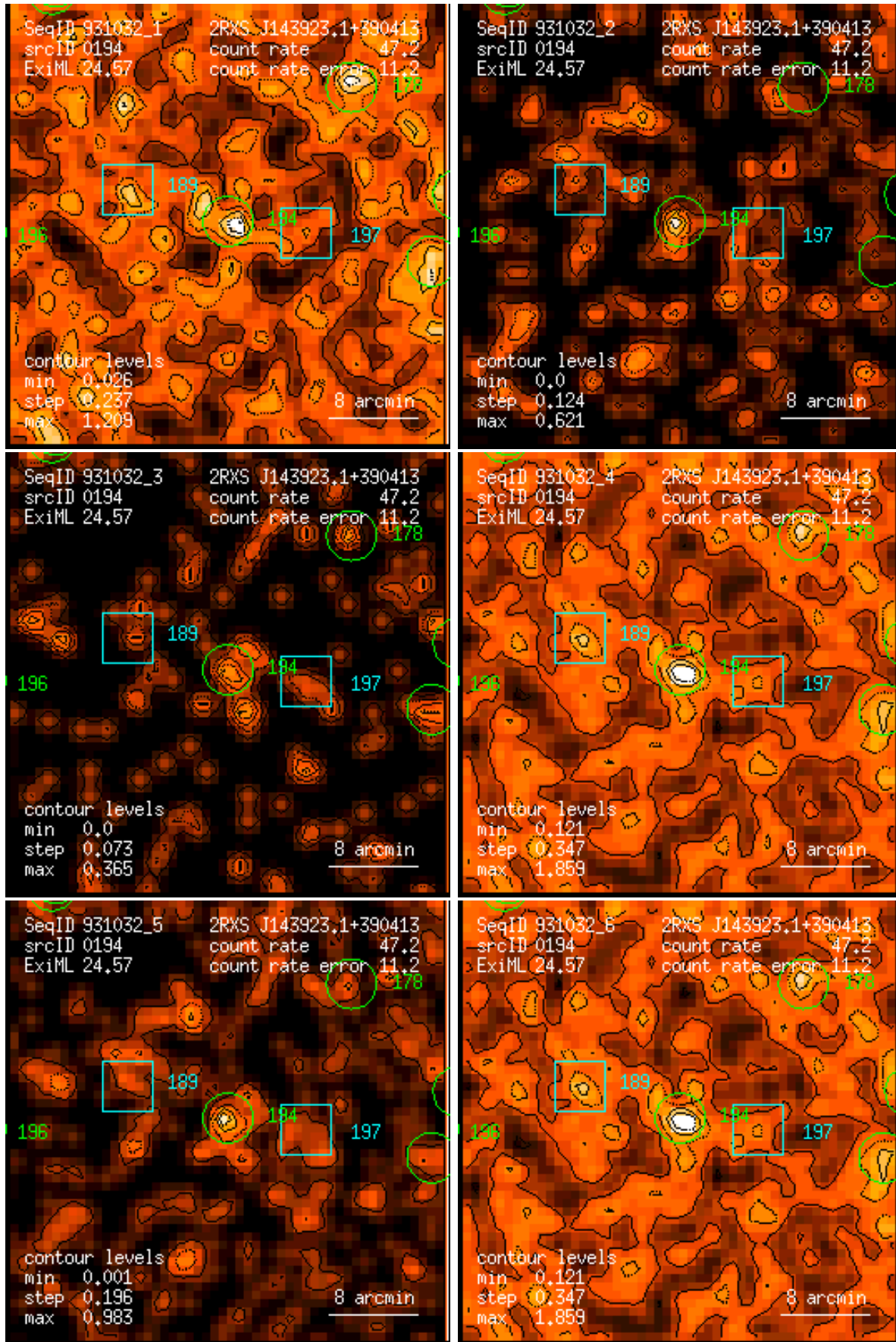
Figure 194: RASS 931032: detection 0194: band rate images, Gaussian filter: (1) PSPC channels 11 – 41, (2) 52 – 90, (3) 91 – 201, (4) 11 – 235, (5) 52 – 201, (6) 11 – 201. Broad band rates in counts/ks. Band rate contour levels in counts/ks/arcmin 2 .
