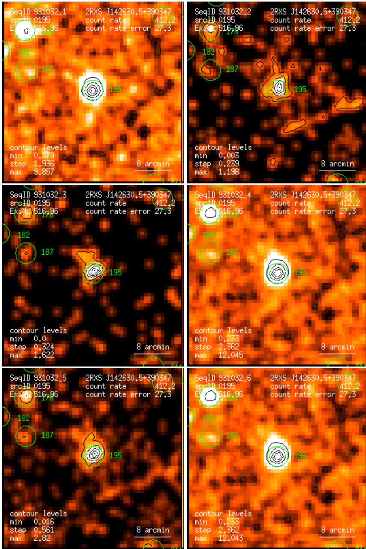
Figure 195: RASS 931032: detection 0195: band rate images, Gaussian filter: (1) PSPC channels 11 – 41, (2) 52 – 90, (3) 91 – 201, (4) 11 – 235, (5) 52 – 201, (6) 11 – 201. Broad band rates in counts/ks. Band rate contour levels in counts/ks/arcmin 2 .
