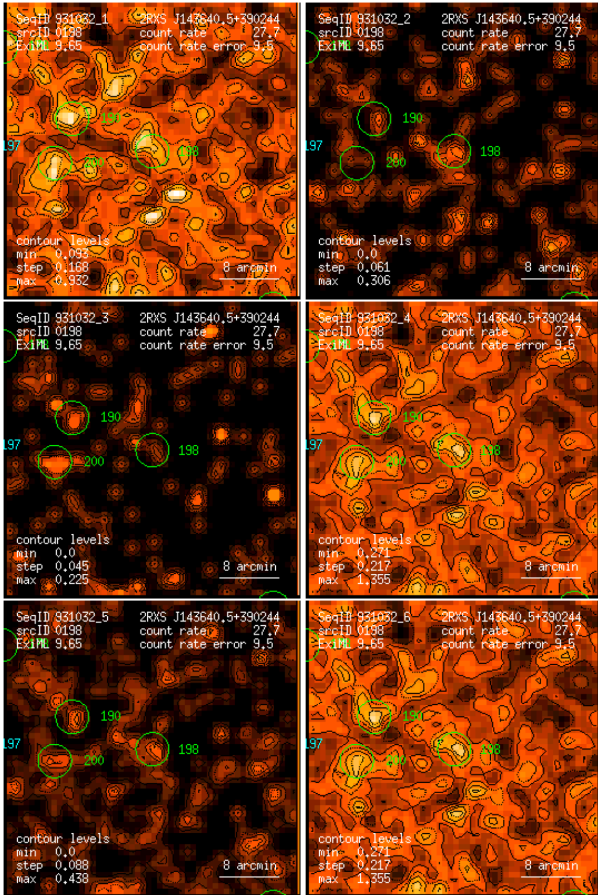
Figure 198: RASS 931032: detection 0198: band rate images, Gaussian filter: (1) PSPC channels 11 – 41, (2) 52 – 90, (3) 91 – 201, (4) 11 – 235, (5) 52 – 201, (6) 11 – 201. Broad band rates in counts/ks. Band rate contour levels in counts/ks/arcmin 2 .
