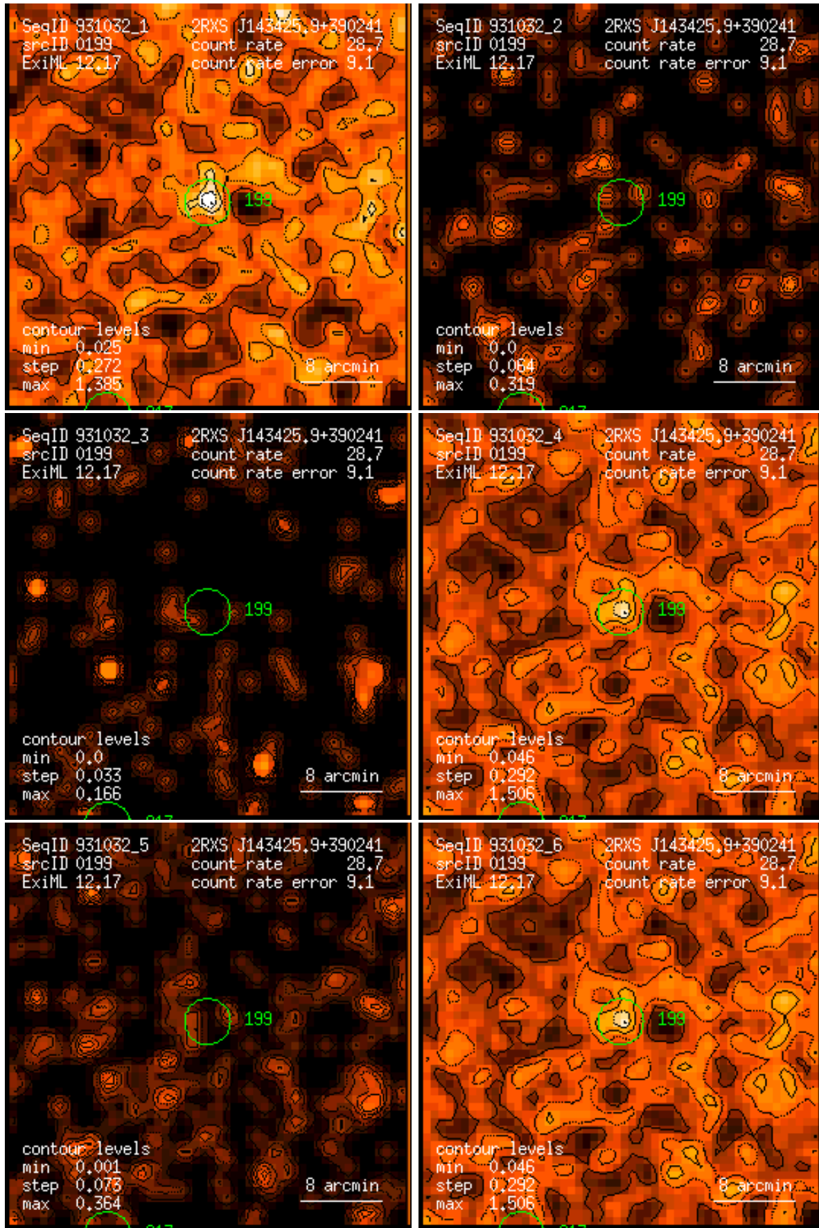
Figure 199: RASS 931032: detection 0199: band rate images, Gaussian filter: (1) PSPC channels 11 – 41, (2) 52 – 90, (3) 91 – 201, (4) 11 – 235, (5) 52 – 201, (6) 11 – 201. Broad band rates in counts/ks. Band rate contour levels in counts/ks/arcmin 2 .
