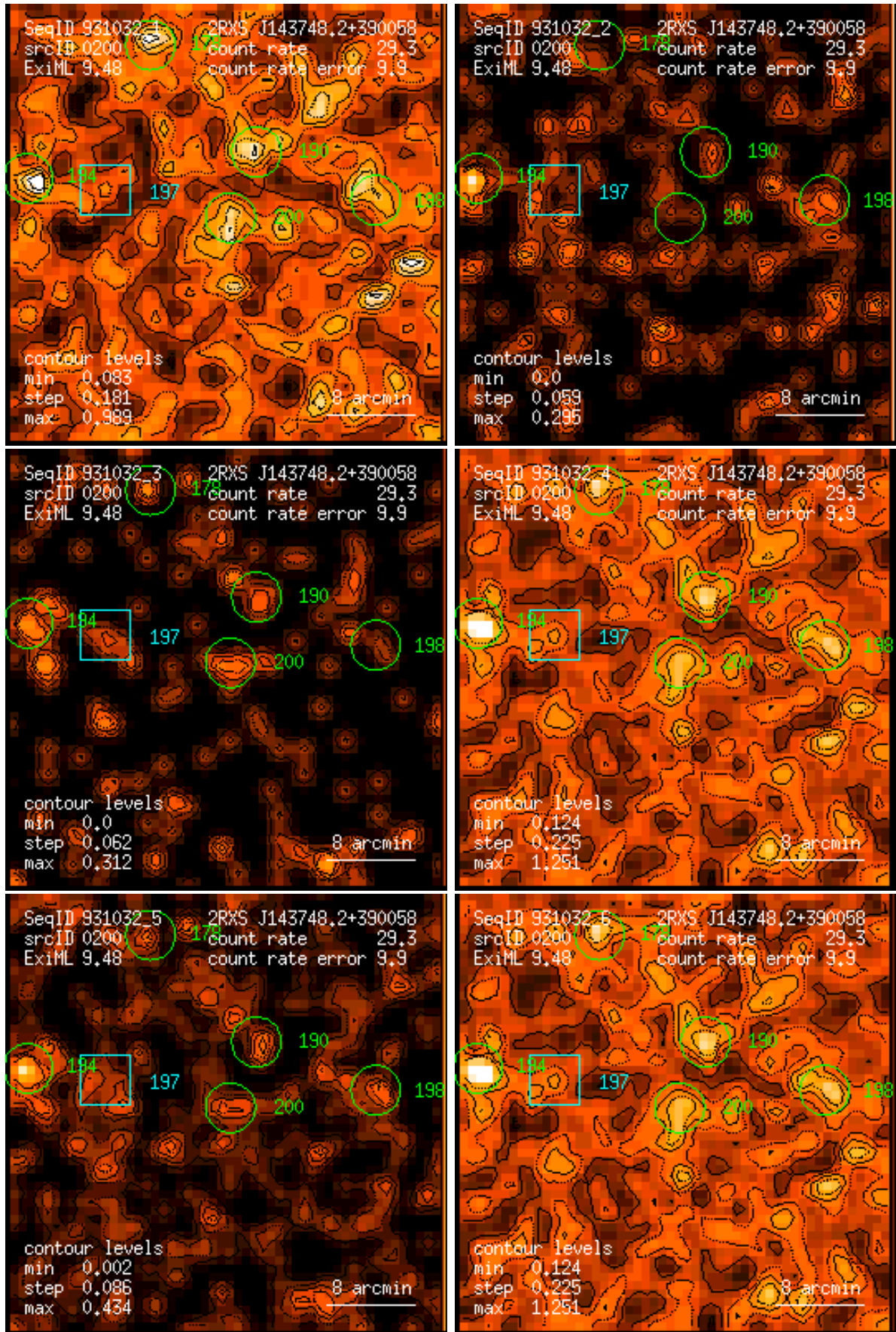
Figure 200: RASS 931032: detection 0200: band rate images, Gaussian filter: (1) PSPC channels 11 – 41, (2) 52 – 90, (3) 91 – 201, (4) 11 – 235, (5) 52 – 201, (6) 11 – 201. Broad band rates in counts/ks. Band rate contour levels in counts/ks/arcmin 2 .
