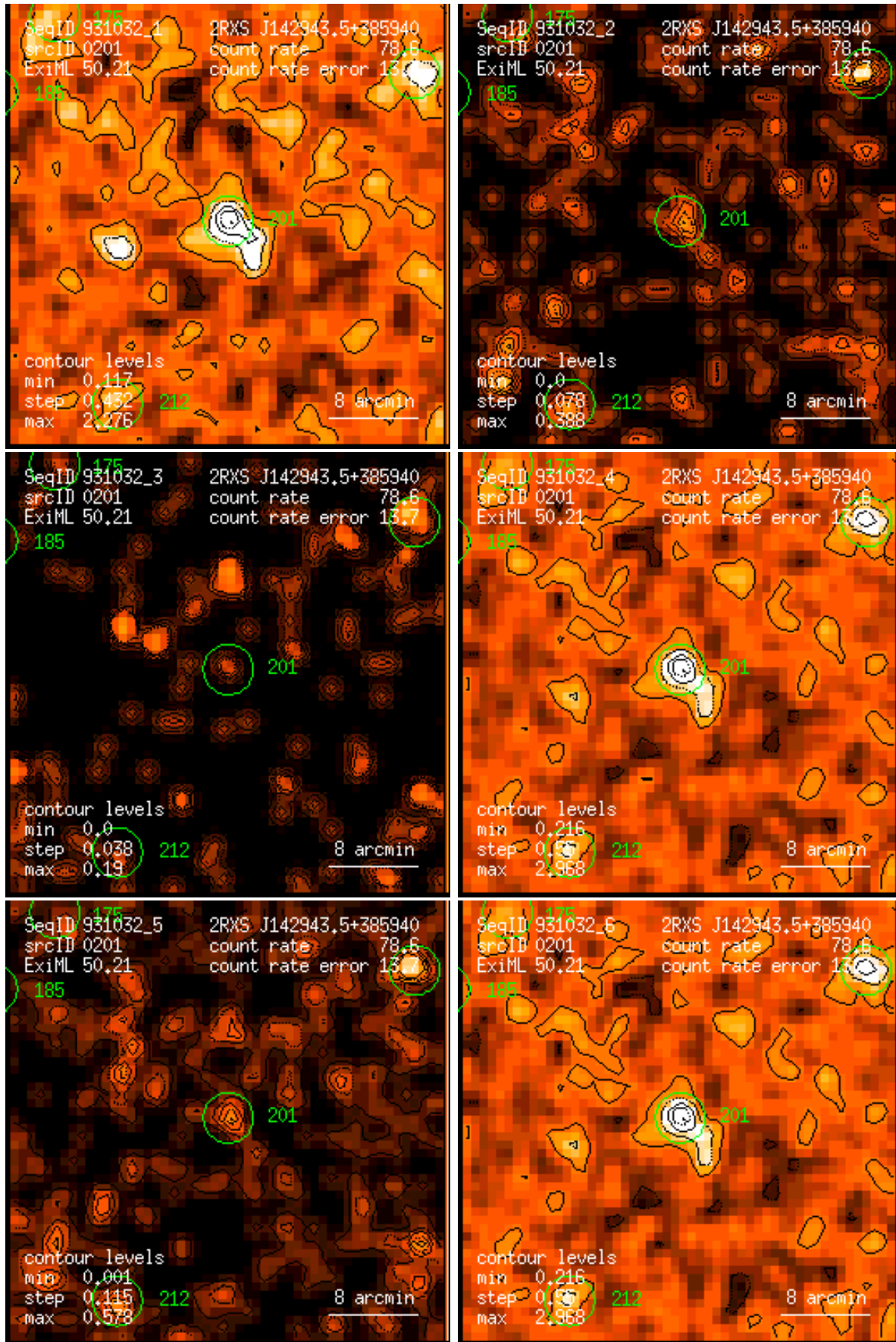
Figure 201: RASS 931032: detection 0201: band rate images, Gaussian filter: (1) PSPC channels 11 – 41, (2) 52 – 90, (3) 91 – 201, (4) 11 – 235, (5) 52 – 201, (6) 11 – 201. Broad band rates in counts/ks. Band rate contour levels in counts/ks/arcmin 2 .
