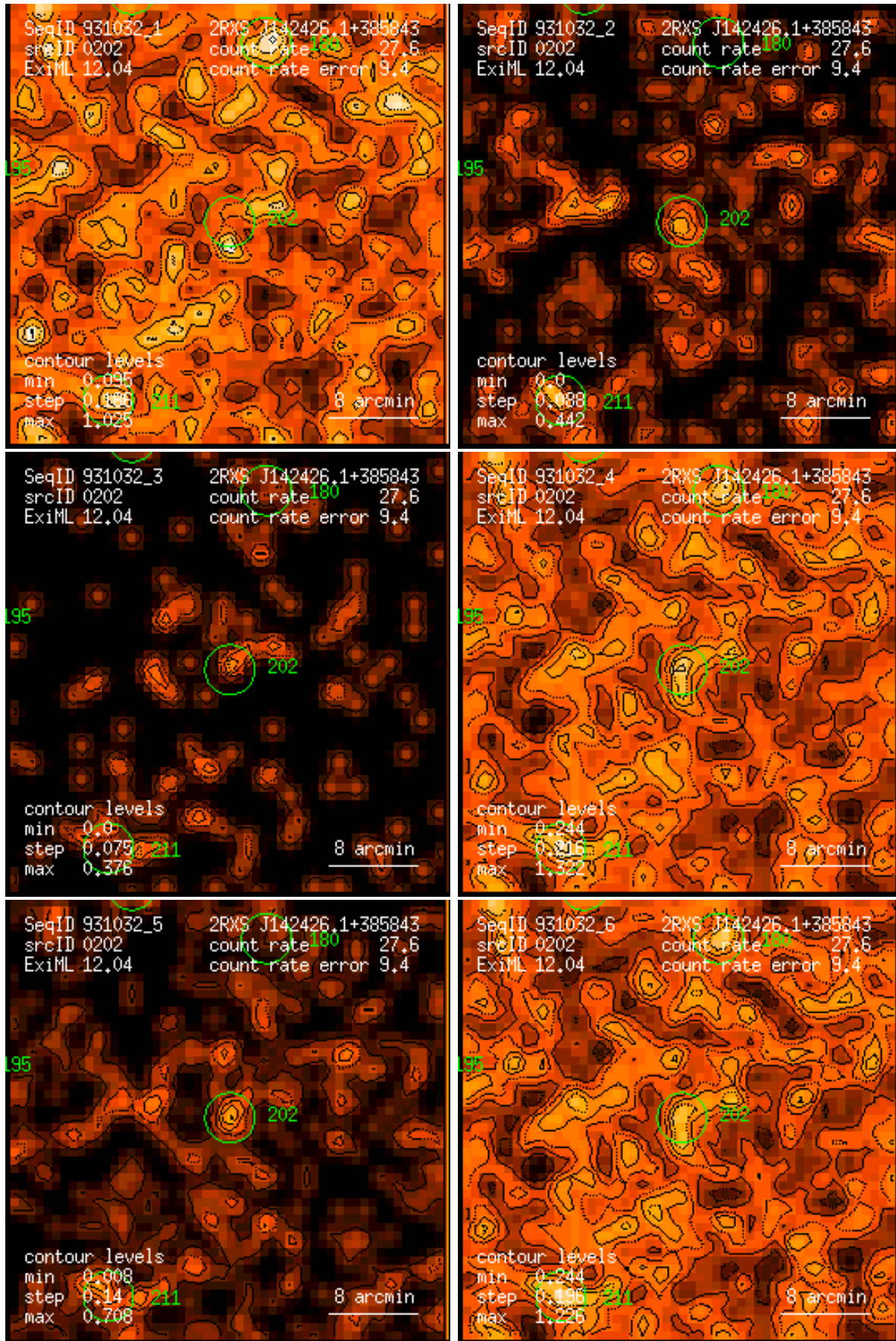
Figure 202: RASS 931032: detection 0202: band rate images, Gaussian filter: (1) PSPC channels 11 – 41, (2) 52 – 90, (3) 91 – 201, (4) 11 – 235, (5) 52 – 201, (6) 11 – 201. Broad band rates in counts/ks. Band rate contour levels in counts/ks/arcmin 2 .
