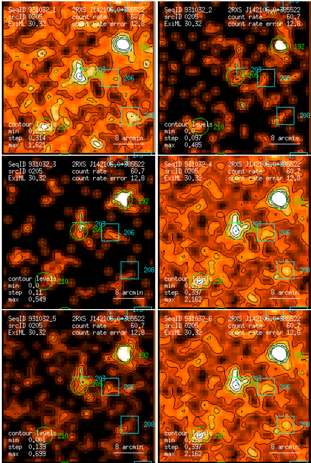
Figure 205: RASS 931032: detection 0205: band rate images, Gaussian filter: (1) PSPC channels 11 – 41, (2) 52 – 90, (3) 91 – 201, (4) 11 – 235, (5) 52 – 201, (6) 11 – 201. Broad band rates in counts/ks. Band rate contour levels in counts/ks/arcmin 2 .
