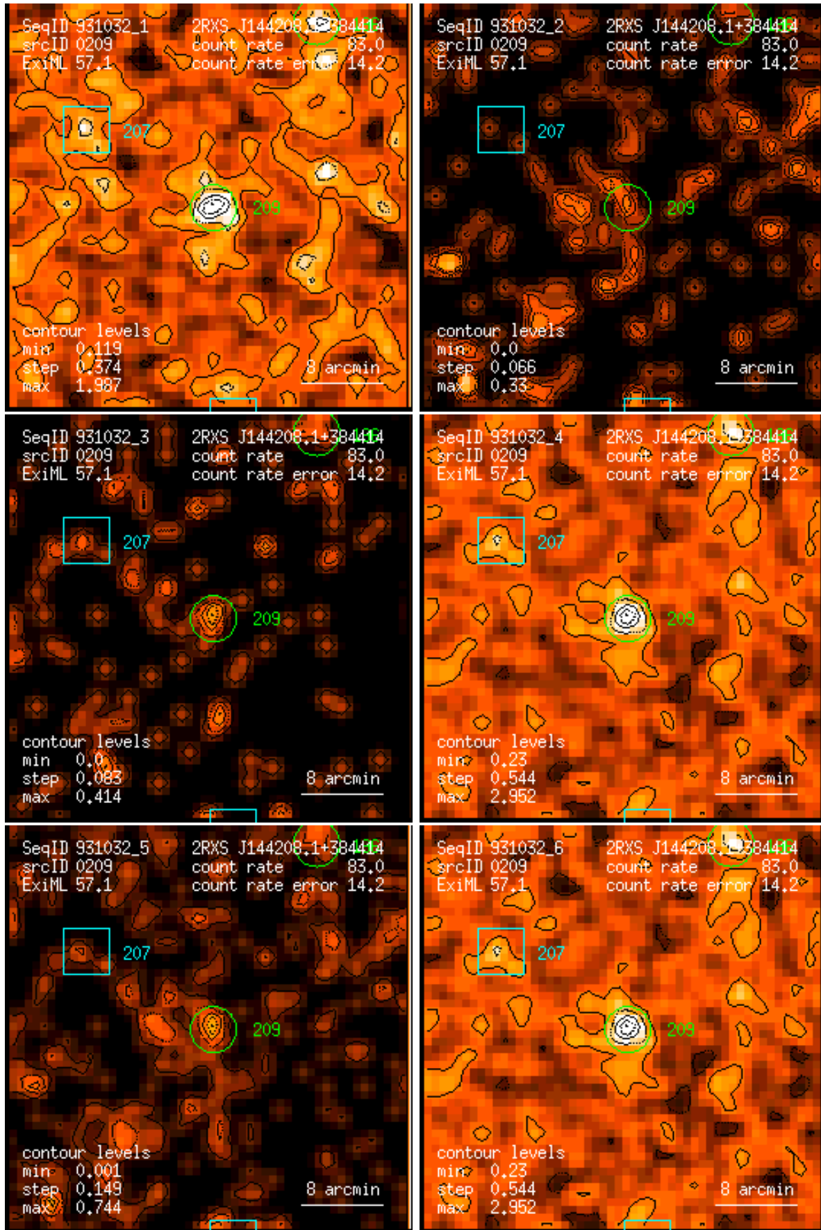
Figure 209: RASS 931032: detection 0209: band rate images, Gaussian filter: (1) PSPC channels 11 – 41, (2) 52 – 90, (3) 91 – 201, (4) 11 – 235, (5) 52 – 201, (6) 11 – 201. Broad band rates in counts/ks. Band rate contour levels in counts/ks/arcmin 2 .
