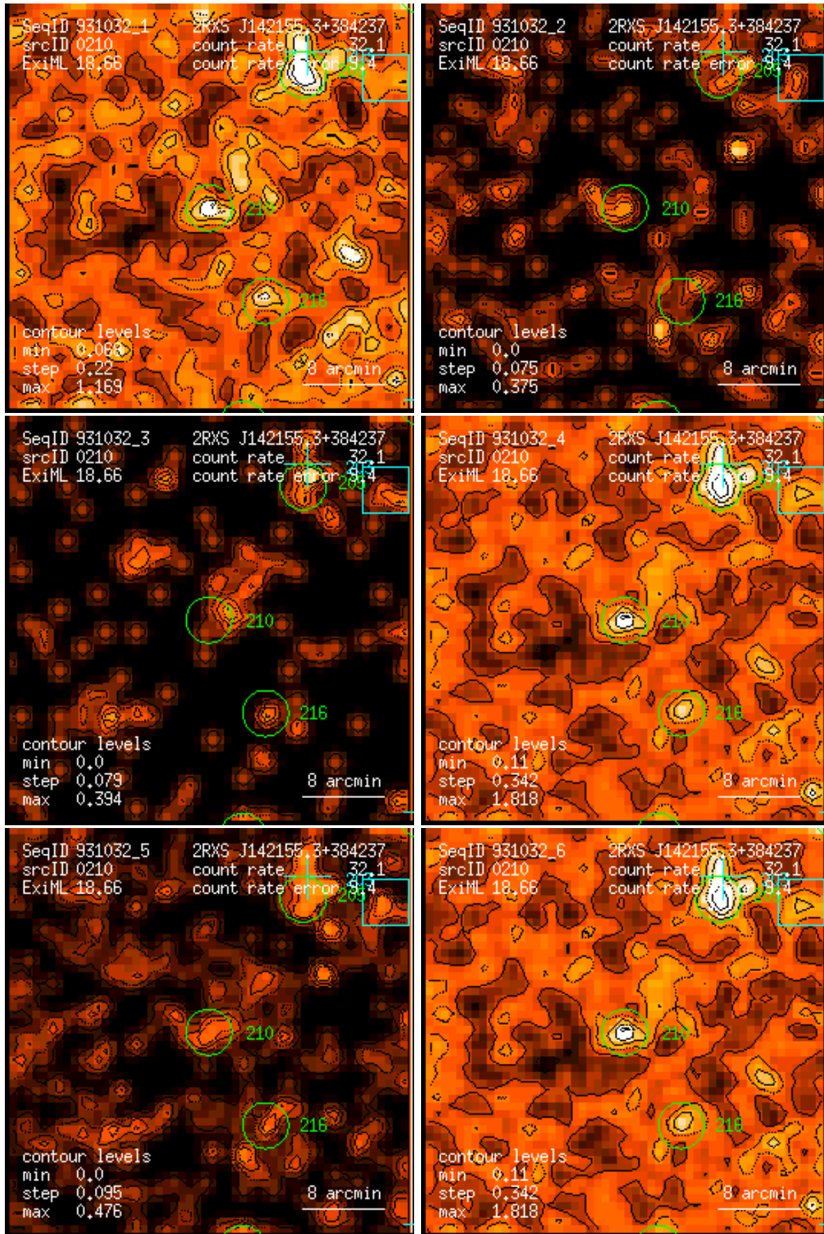
Figure 210: RASS 931032: detection 0210: band rate images, Gaussian filter: (1) PSPC channels 11 – 41, (2) 52 – 90, (3) 91 – 201, (4) 11 – 235, (5) 52 – 201, (6) 11 – 201. Broad band rates in counts/ks. Band rate contour levels in counts/ks/arcmin 2 .
