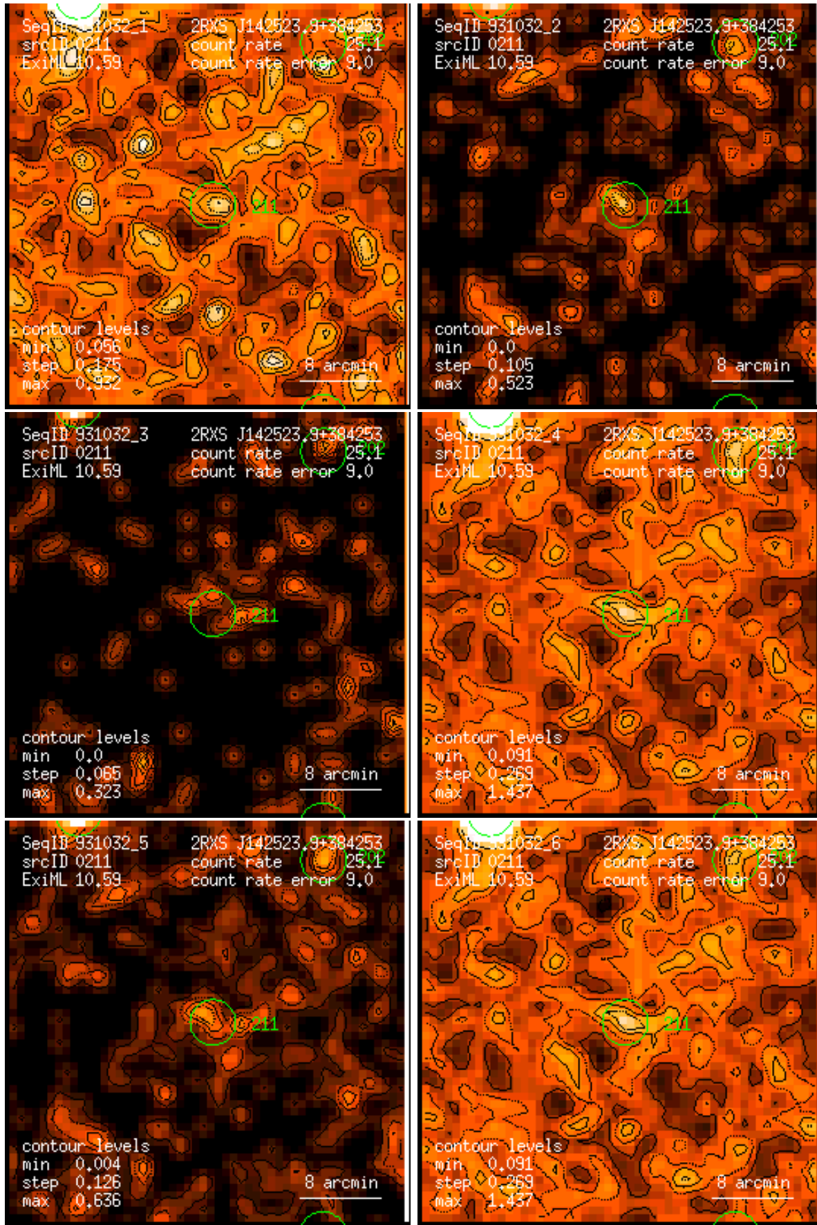
Figure 211: RASS 931032: detection 0211: band rate images, Gaussian filter: (1) PSPC channels 11 – 41, (2) 52 – 90, (3) 91 – 201, (4) 11 – 235, (5) 52 – 201, (6) 11 – 201. Broad band rates in counts/ks. Band rate contour levels in counts/ks/arcmin 2 .
