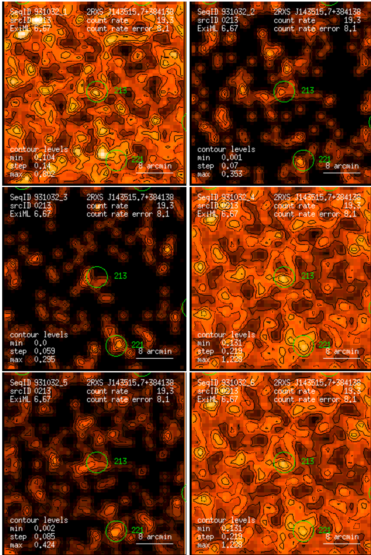
Figure 213: RASS 931032: detection 0213: band rate images, Gaussian filter: (1) PSPC channels 11 – 41, (2) 52 – 90, (3) 91 – 201, (4) 11 – 235, (5) 52 – 201, (6) 11 – 201. Broad band rates in counts/ks. Band rate contour levels in counts/ks/arcmin 2 .
