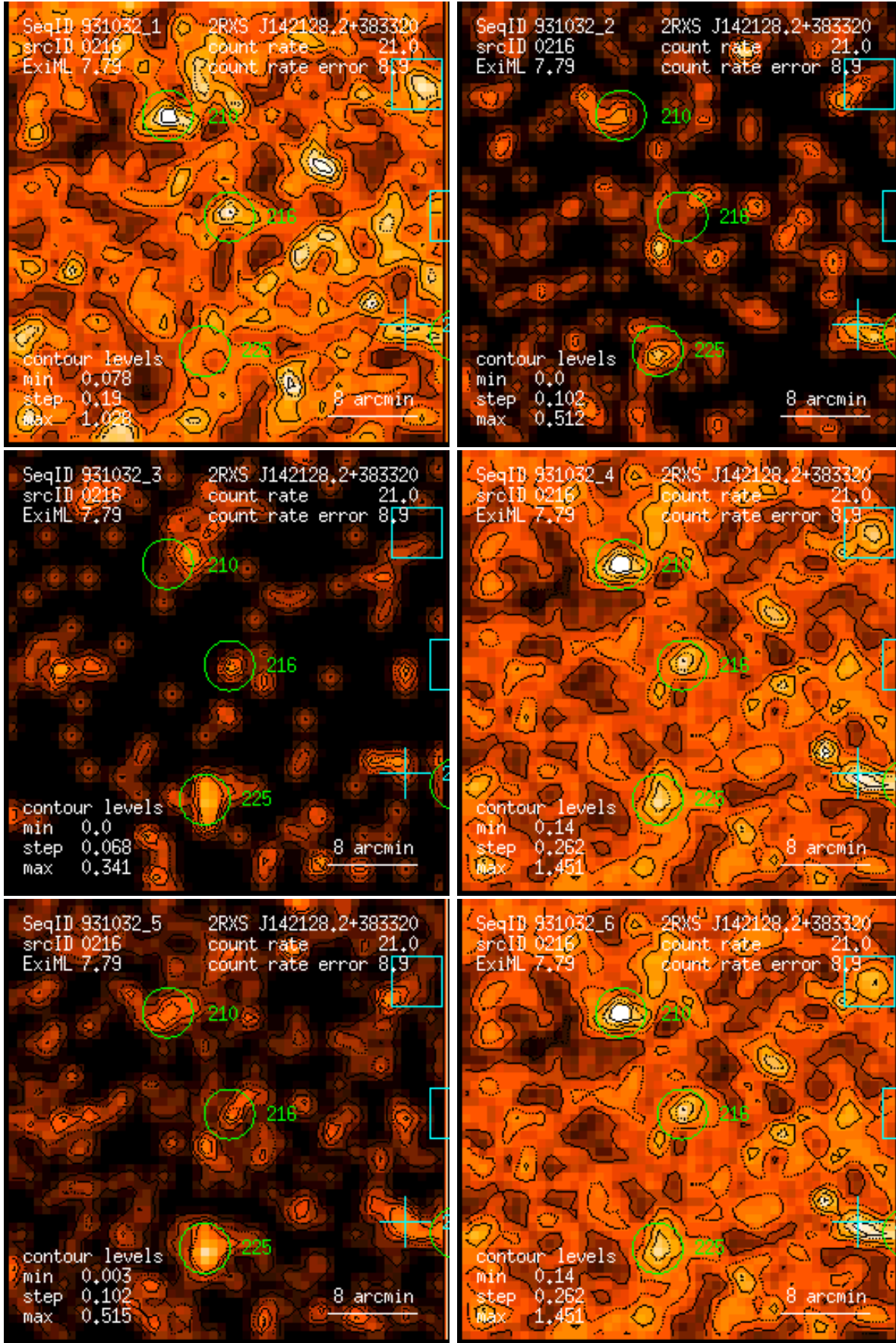
Figure 216: RASS 931032: detection 0216: band rate images, Gaussian filter: (1) PSPC channels 11 – 41, (2) 52 – 90, (3) 91 – 201, (4) 11 – 235, (5) 52 – 201, (6) 11 – 201. Broad band rates in counts/ks. Band rate contour levels in counts/ks/arcmin 2 .
