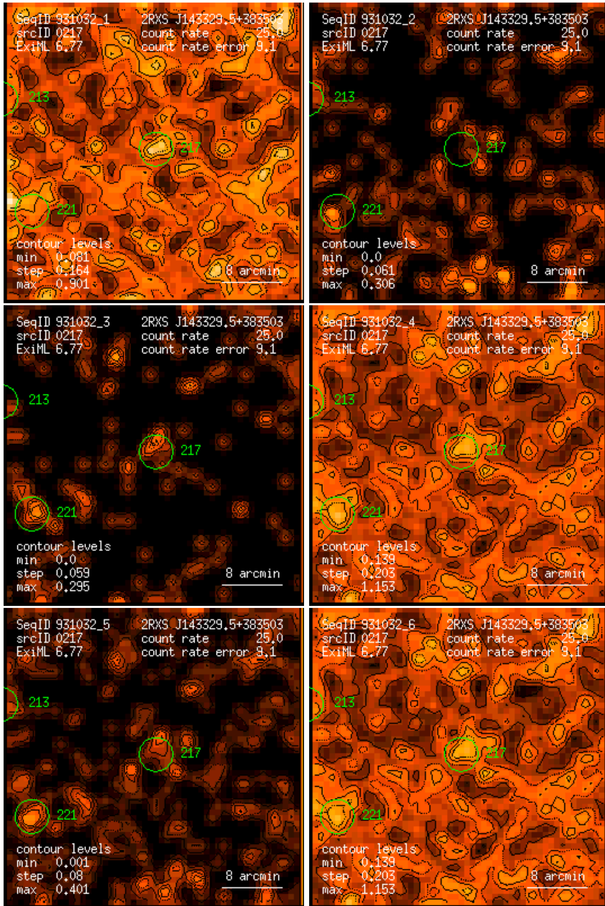
Figure 217: RASS 931032: detection 0217: band rate images, Gaussian filter: (1) PSPC channels 11 – 41, (2) 52 – 90, (3) 91 – 201, (4) 11 – 235, (5) 52 – 201, (6) 11 – 201. Broad band rates in counts/ks. Band rate contour levels in counts/ks/arcmin 2 .
