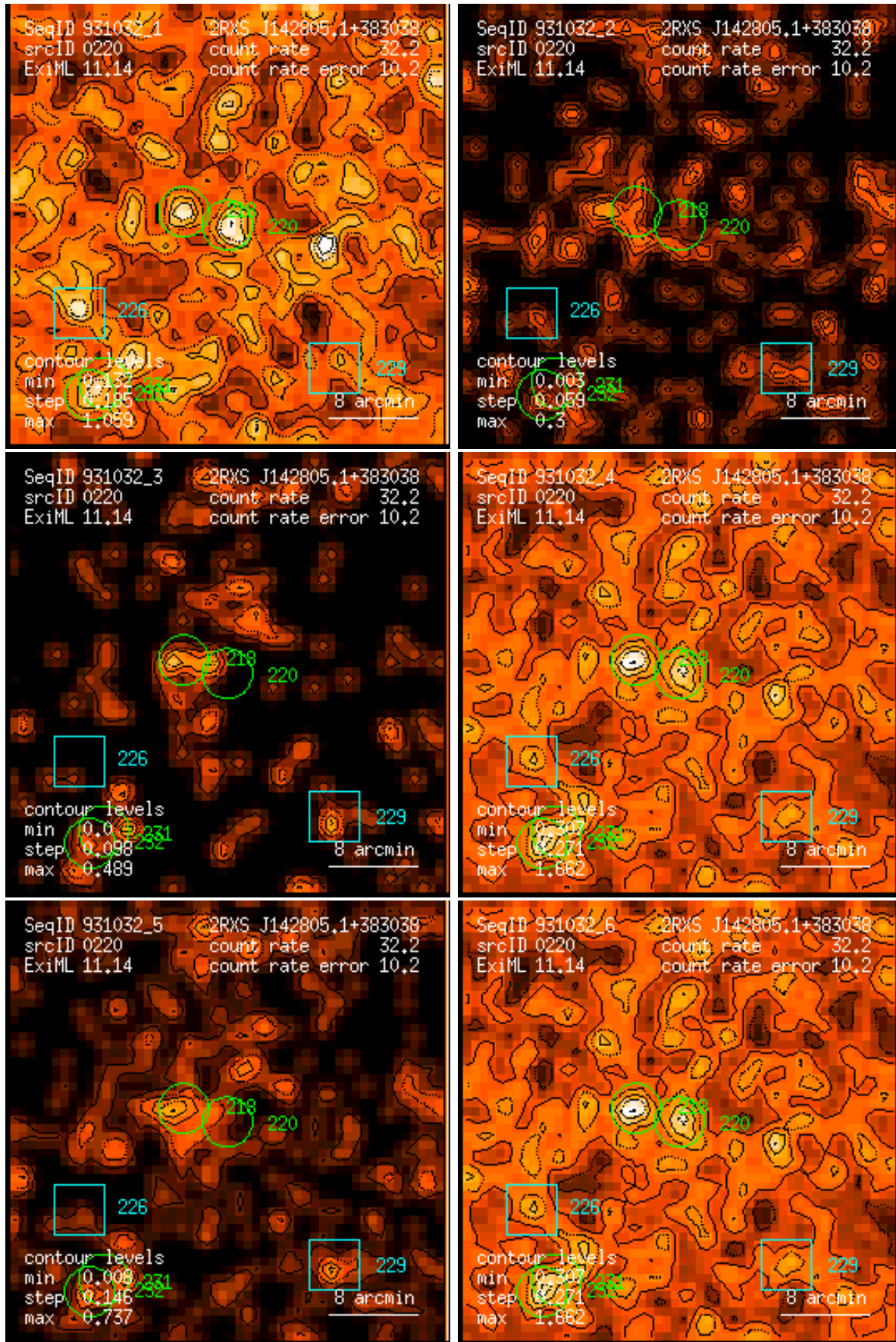
Figure 220: RASS 931032: detection 0220: band rate images, Gaussian filter: (1) PSPC channels 11 – 41, (2) 52 – 90, (3) 91 – 201, (4) 11 – 235, (5) 52 – 201, (6) 11 – 201. Broad band rates in counts/ks. Band rate contour levels in counts/ks/arcmin 2 .
