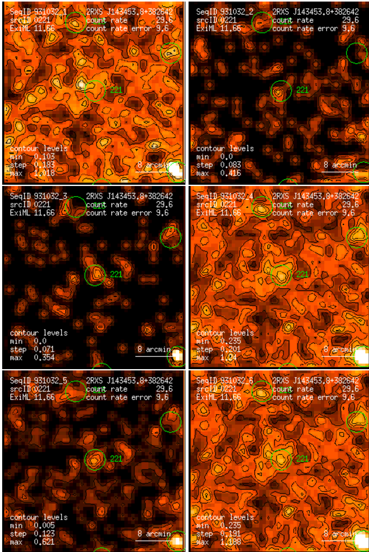
Figure 221: RASS 931032: detection 0221: band rate images, Gaussian filter: (1) PSPC channels 11 – 41, (2) 52 – 90, (3) 91 – 201, (4) 11 – 235, (5) 52 – 201, (6) 11 – 201. Broad band rates in counts/ks. Band rate contour levels in counts/ks/arcmin 2 .
