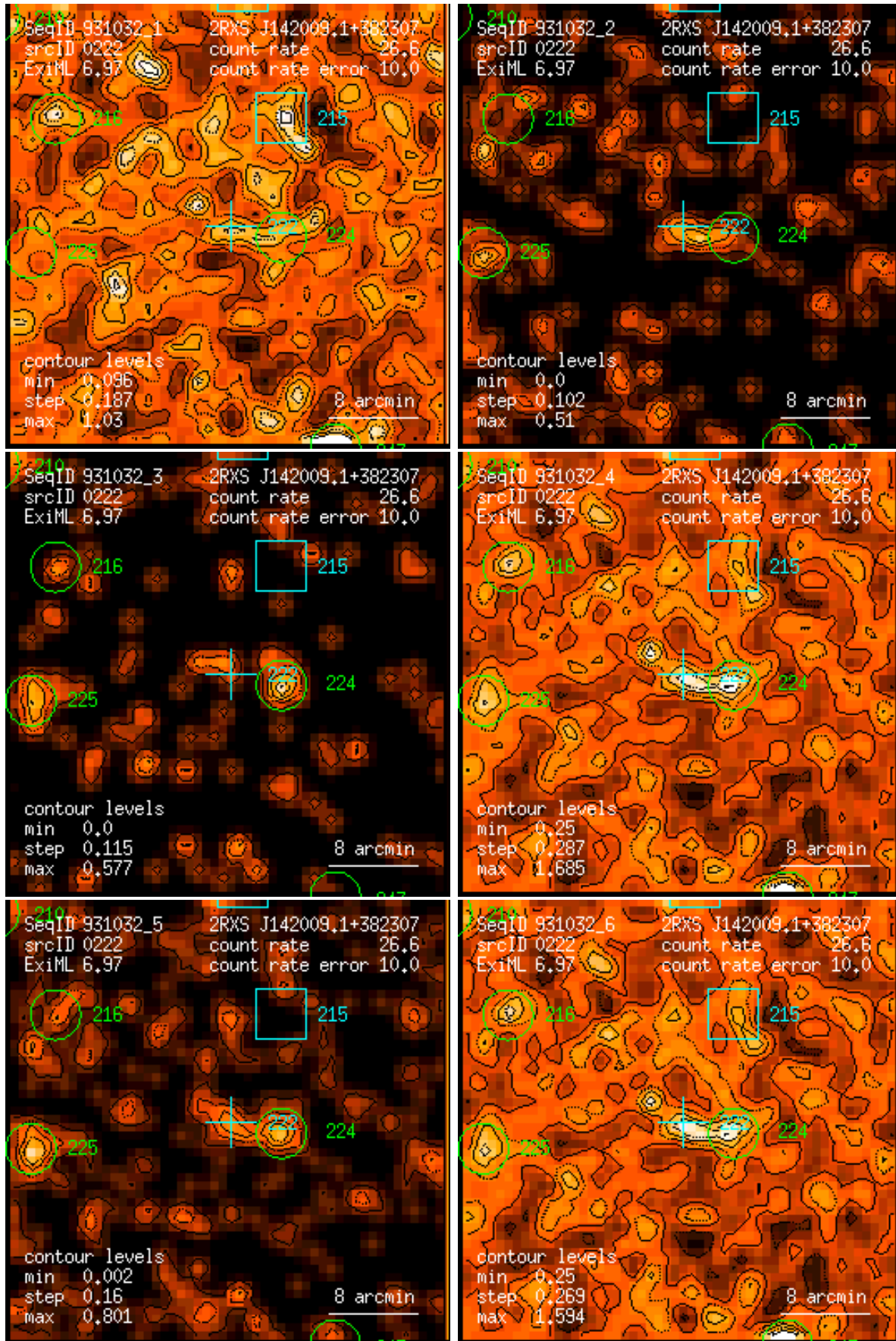
Figure 222: RASS 931032: detection 0222: band rate images, Gaussian filter: (1) PSPC channels 11 – 41, (2) 52 – 90, (3) 91 – 201, (4) 11 – 235, (5) 52 – 201, (6) 11 – 201. Broad band rates in counts/ks. Band rate contour levels in counts/ks/arcmin 2 .
