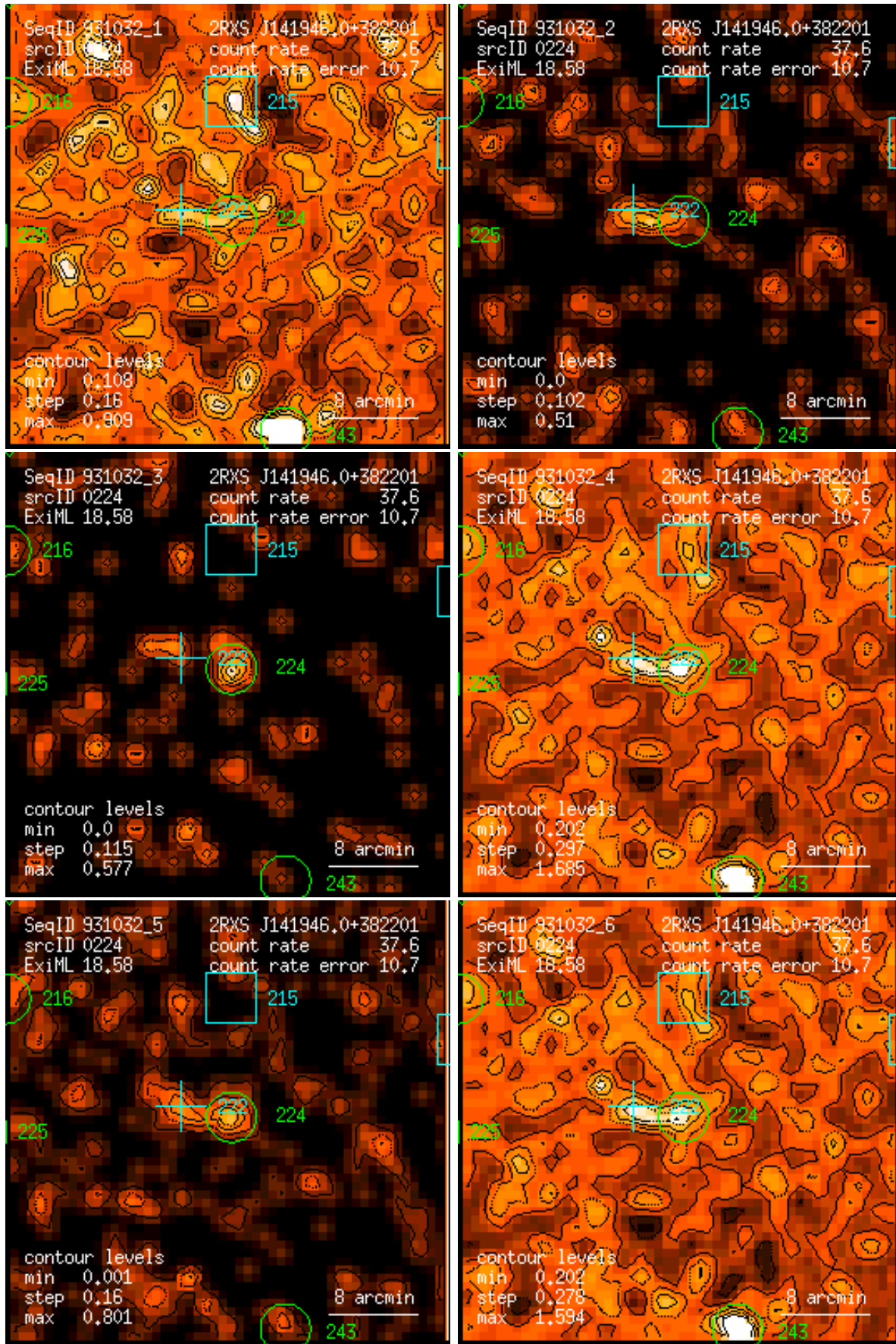
Figure 224: RASS 931032: detection 0224: band rate images, Gaussian filter: (1) PSPC channels 11 – 41, (2) 52 – 90, (3) 91 – 201, (4) 11 – 235, (5) 52 – 201, (6) 11 – 201. Broad band rates in counts/ks. Band rate contour levels in counts/ks/arcmin 2 .
