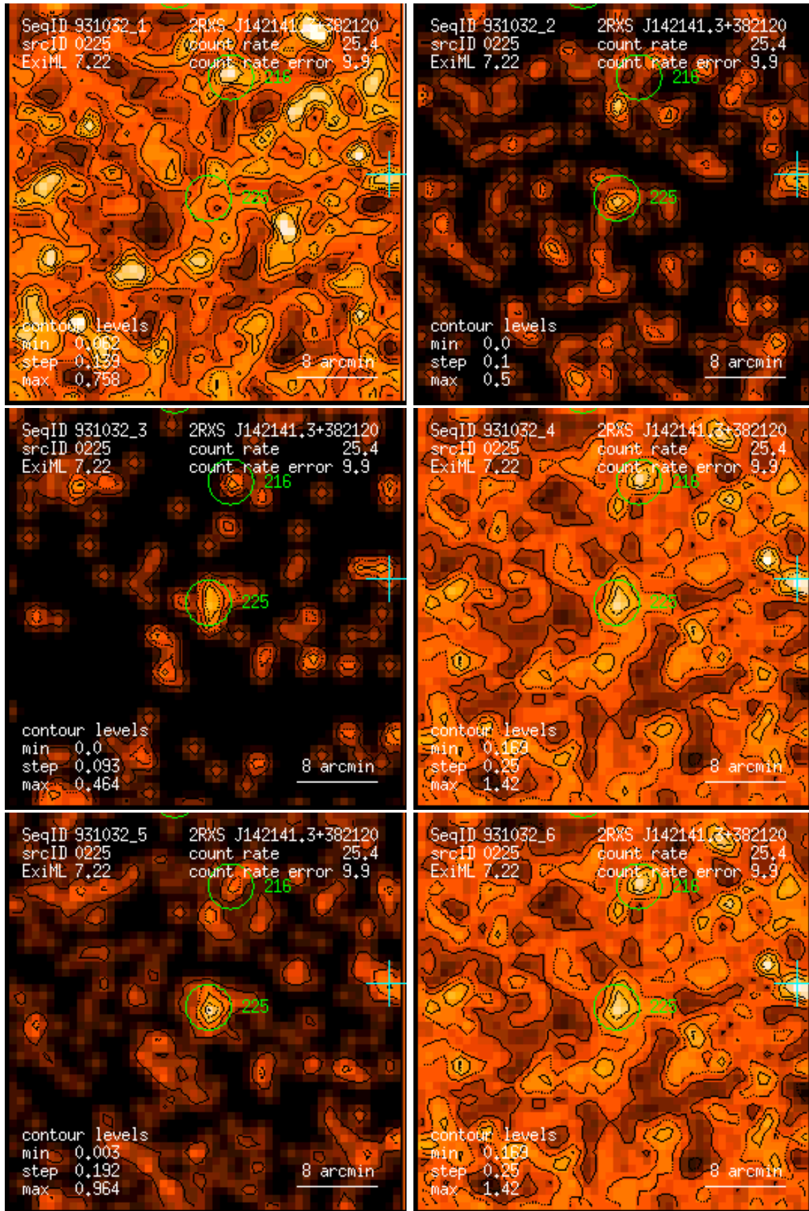
Figure 225: RASS 931032: detection 0225: band rate images, Gaussian filter: (1) PSPC channels 11 – 41, (2) 52 – 90, (3) 91 – 201, (4) 11 – 235, (5) 52 – 201, (6) 11 – 201. Broad band rates in counts/ks. Band rate contour levels in counts/ks/arcmin 2 .
