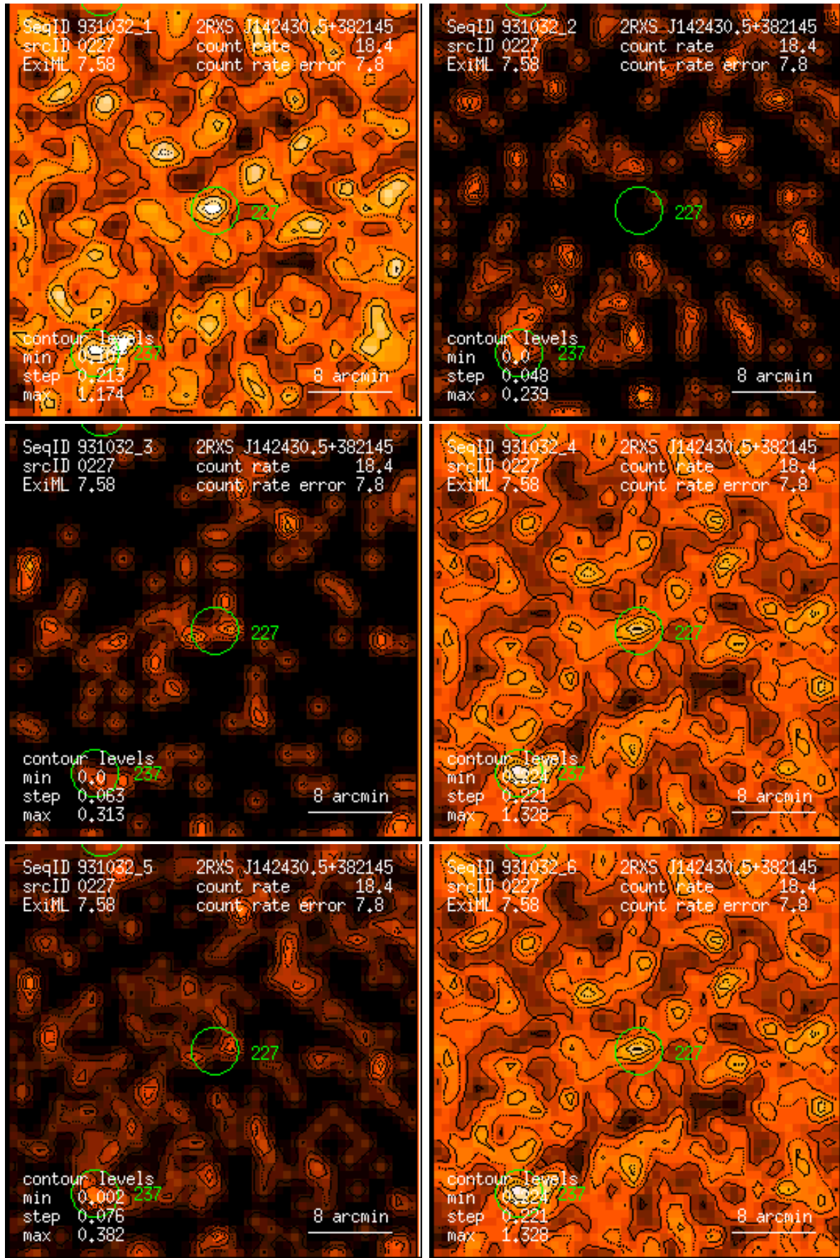
Figure 227: RASS 931032: detection 0227: band rate images, Gaussian filter: (1) PSPC channels 11 – 41, (2) 52 – 90, (3) 91 – 201, (4) 11 – 235, (5) 52 – 201, (6) 11 – 201. Broad band rates in counts/ks. Band rate contour levels in counts/ks/arcmin 2 .
