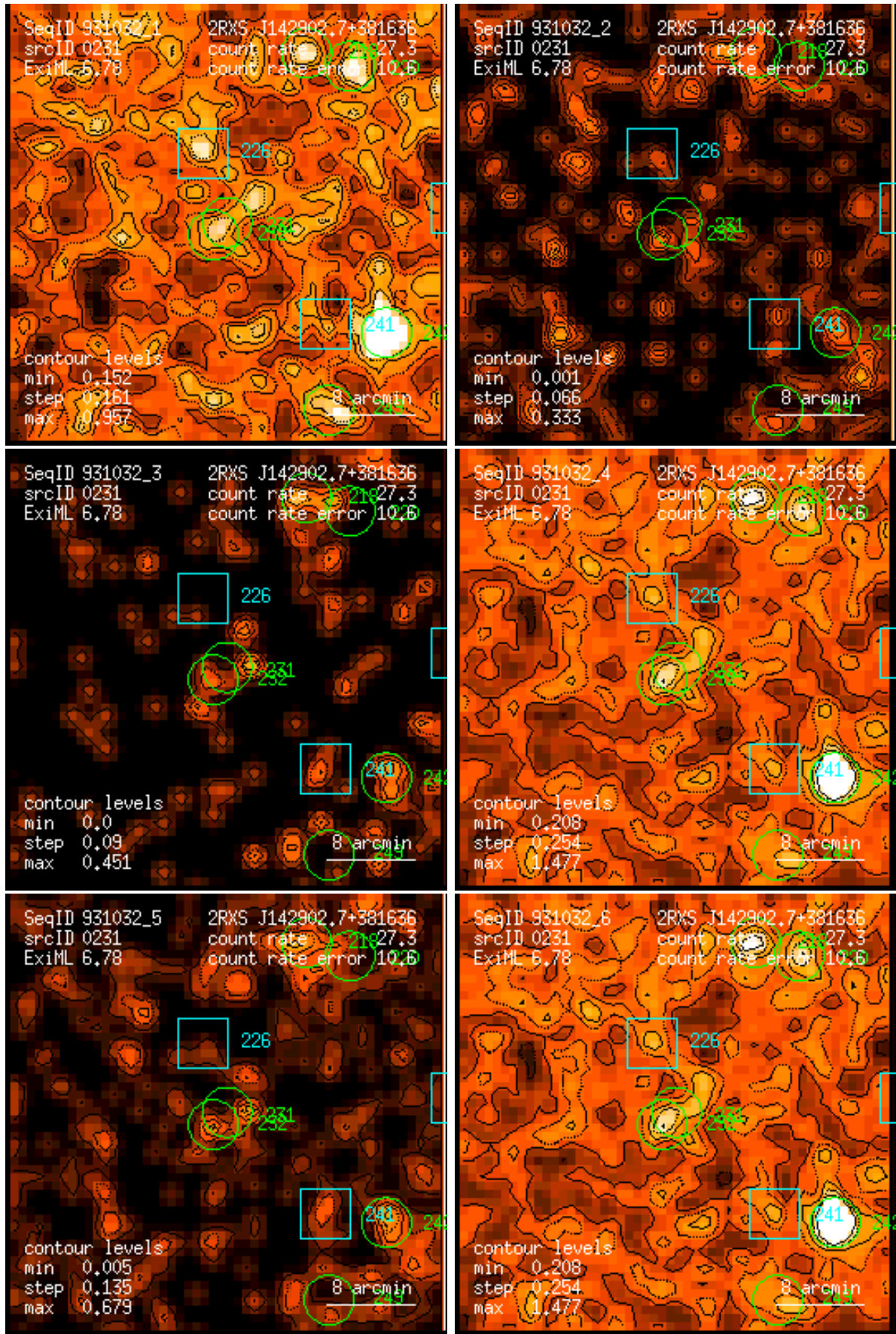
Figure 231: RASS 931032: detection 0231: band rate images, Gaussian filter: (1) PSPC channels 11 – 41, (2) 52 – 90, (3) 91 – 201, (4) 11 – 235, (5) 52 – 201, (6) 11 – 201. Broad band rates in counts/ks. Band rate contour levels in counts/ks/arcmin 2 .
