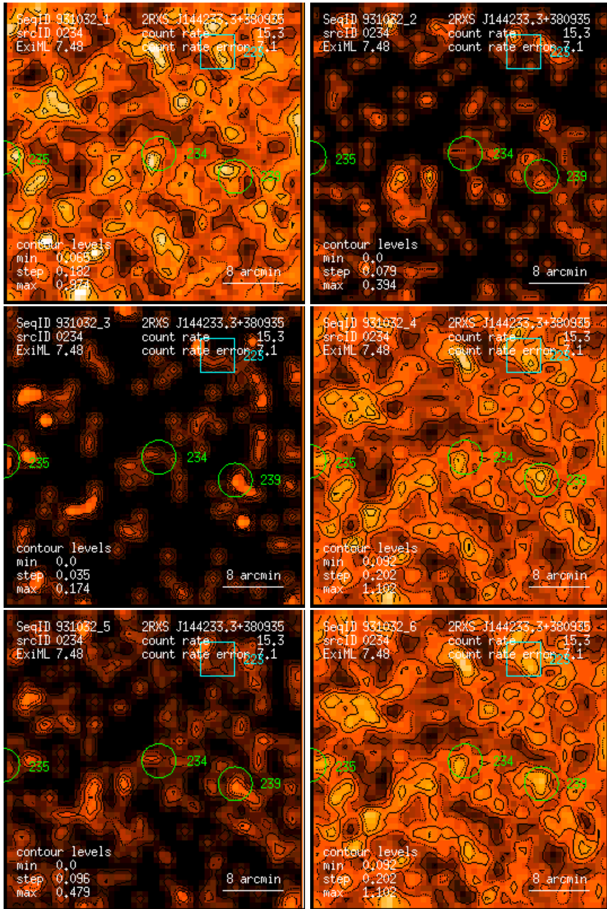
Figure 234: RASS 931032: detection 0234: band rate images, Gaussian filter: (1) PSPC channels 11 – 41, (2) 52 – 90, (3) 91 – 201, (4) 11 – 235, (5) 52 – 201, (6) 11 – 201. Broad band rates in counts/ks. Band rate contour levels in counts/ks/arcmin 2 .
