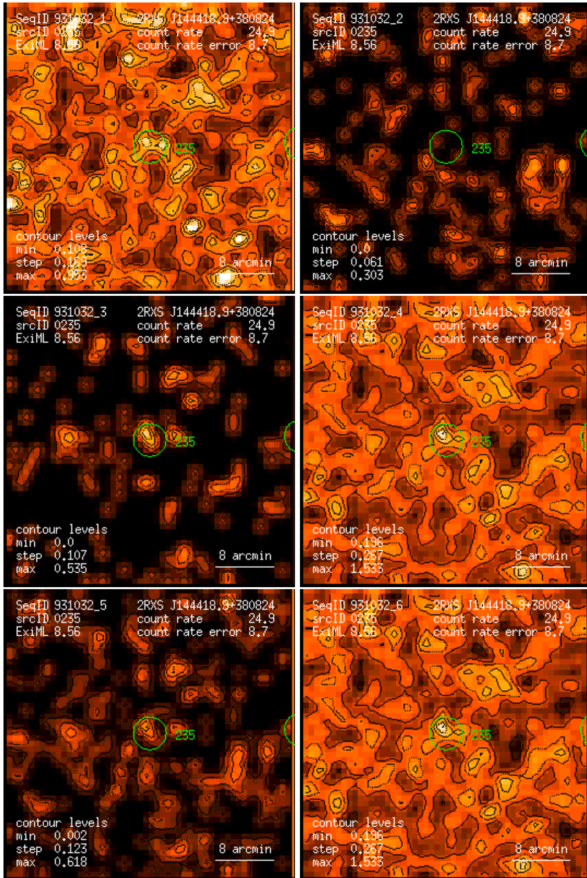
Figure 235: RASS 931032: detection 0235: band rate images, Gaussian filter: (1) PSPC channels 11 – 41, (2) 52 – 90, (3) 91 – 201, (4) 11 – 235, (5) 52 – 201, (6) 11 – 201. Broad band rates in counts/ks. Band rate contour levels in counts/ks/arcmin 2 .
