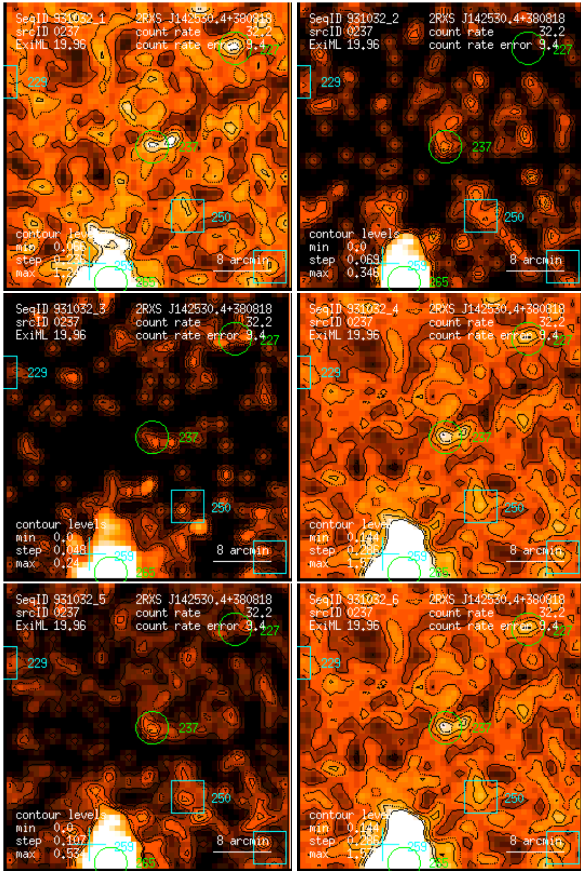
Figure 237: RASS 931032: detection 0237: band rate images, Gaussian filter: (1) PSPC channels 11 – 41, (2) 52 – 90, (3) 91 – 201, (4) 11 – 235, (5) 52 – 201, (6) 11 – 201. Broad band rates in counts/ks. Band rate contour levels in counts/ks/arcmin 2 .
