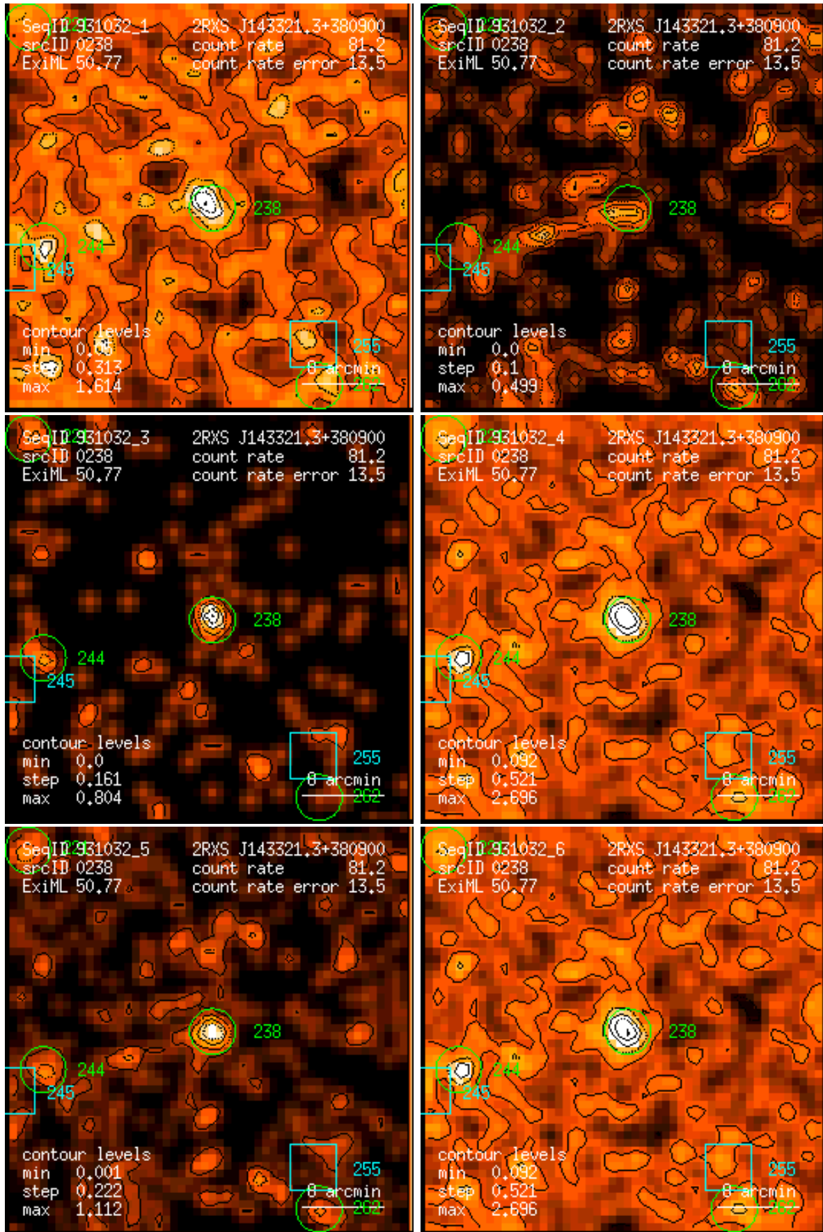
Figure 238: RASS 931032: detection 0238: band rate images, Gaussian filter: (1) PSPC channels 11 – 41, (2) 52 – 90, (3) 91 – 201, (4) 11 – 235, (5) 52 – 201, (6) 11 – 201. Broad band rates in counts/ks. Band rate contour levels in counts/ks/arcmin 2 .
