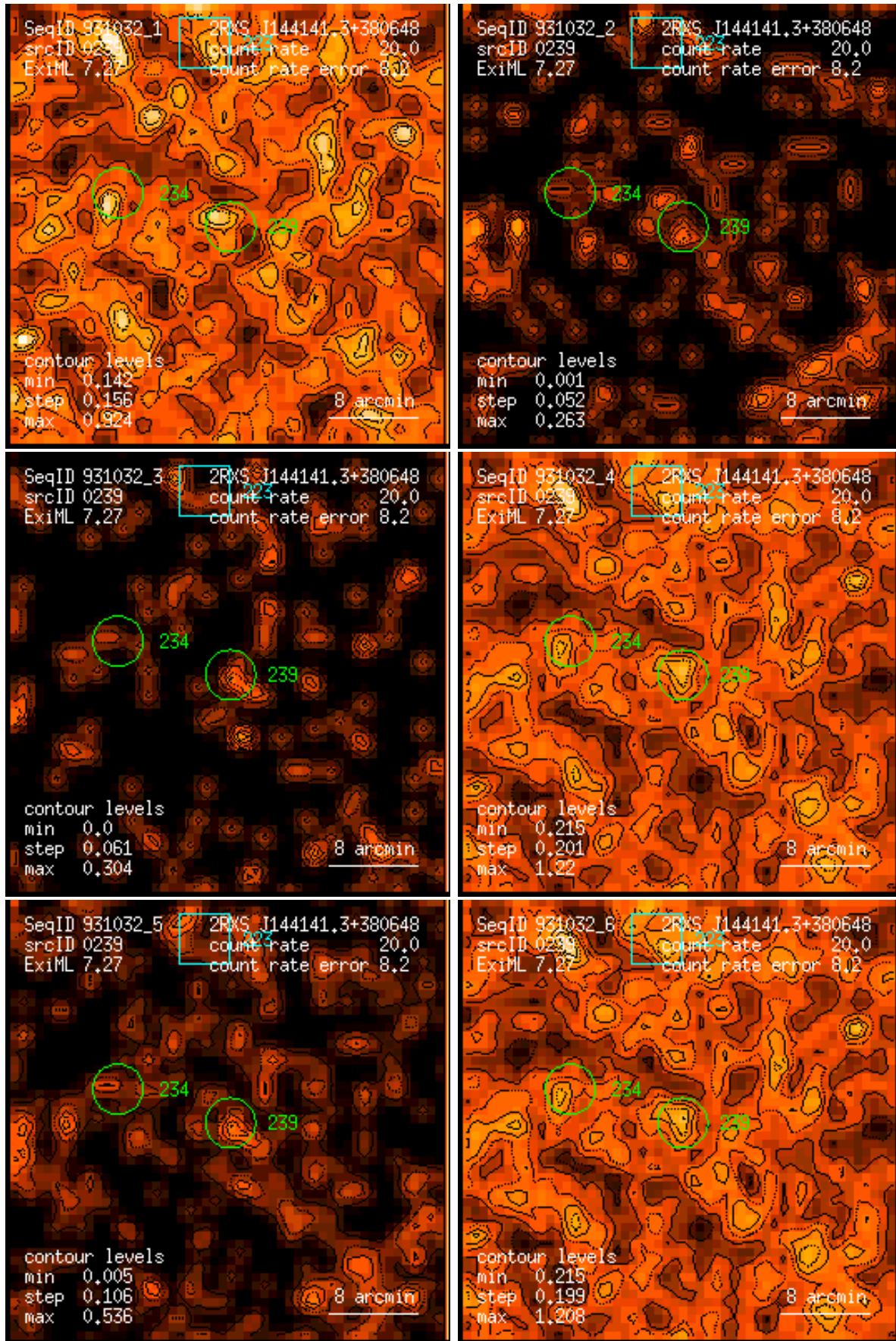
Figure 239: RASS 931032: detection 0239: band rate images, Gaussian filter: (1) PSPC channels 11 – 41, (2) 52 – 90, (3) 91 – 201, (4) 11 – 235, (5) 52 – 201, (6) 11 – 201. Broad band rates in counts/ks. Band rate contour levels in counts/ks/arcmin 2 .
