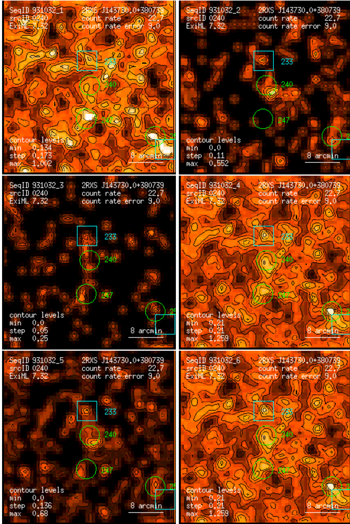
Figure 240: RASS 931032: detection 0240: band rate images, Gaussian filter: (1) PSPC channels 11 – 41, (2) 52 – 90, (3) 91 – 201, (4) 11 – 235, (5) 52 – 201, (6) 11 – 201. Broad band rates in counts/ks. Band rate contour levels in counts/ks/arcmin 2 .
