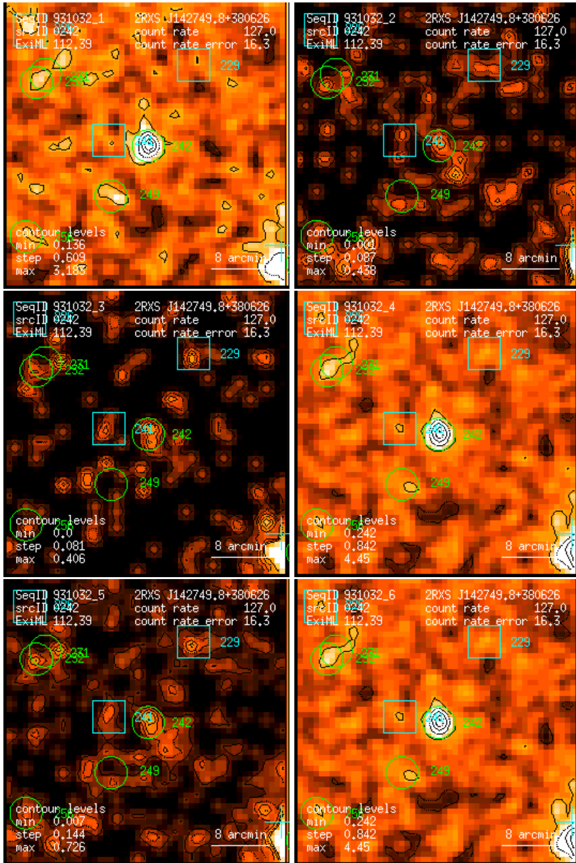
Figure 242: RASS 931032: detection 0242: band rate images, Gaussian filter: (1) PSPC channels 11 – 41, (2) 52 – 90, (3) 91 – 201, (4) 11 – 235, (5) 52 – 201, (6) 11 – 201. Broad band rates in counts/ks. Band rate contour levels in counts/ks/arcmin 2 .
