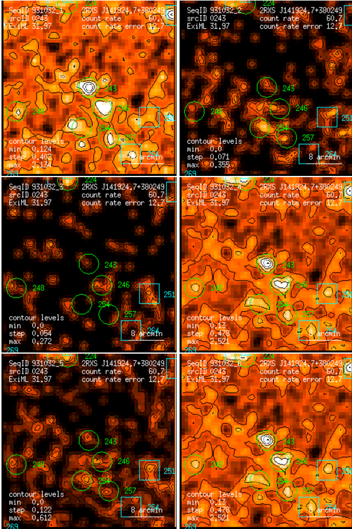
Figure 243: RASS 931032: detection 0243: band rate images, Gaussian filter: (1) PSPC channels 11 – 41, (2) 52 – 90, (3) 91 – 201, (4) 11 – 235, (5) 52 – 201, (6) 11 – 201. Broad band rates in counts/ks. Band rate contour levels in counts/ks/arcmin 2 .
