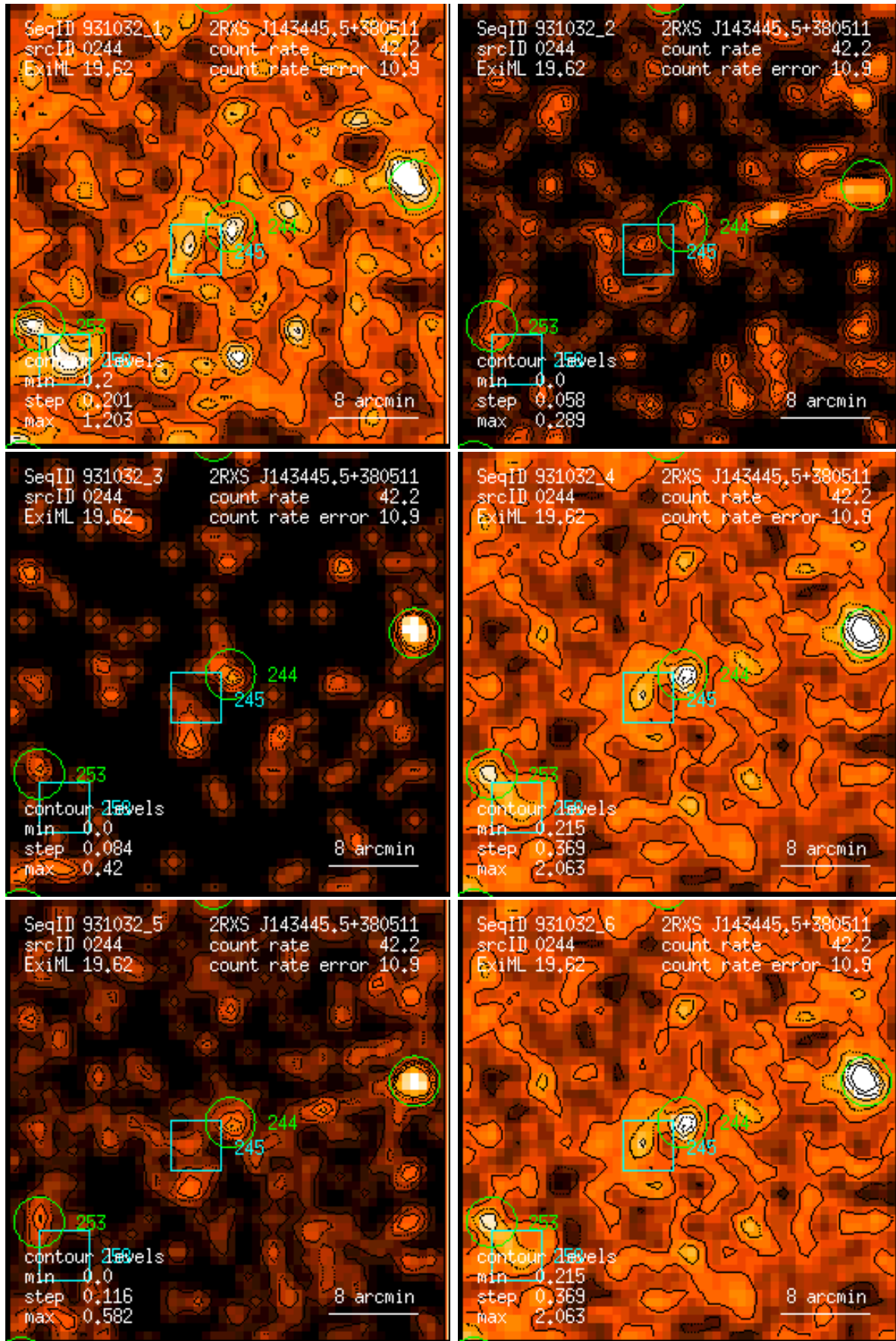
Figure 244: RASS 931032: detection 0244: band rate images, Gaussian filter: (1) PSPC channels 11 – 41, (2) 52 – 90, (3) 91 – 201, (4) 11 – 235, (5) 52 – 201, (6) 11 – 201. Broad band rates in counts/ks. Band rate contour levels in counts/ks/arcmin 2 .
