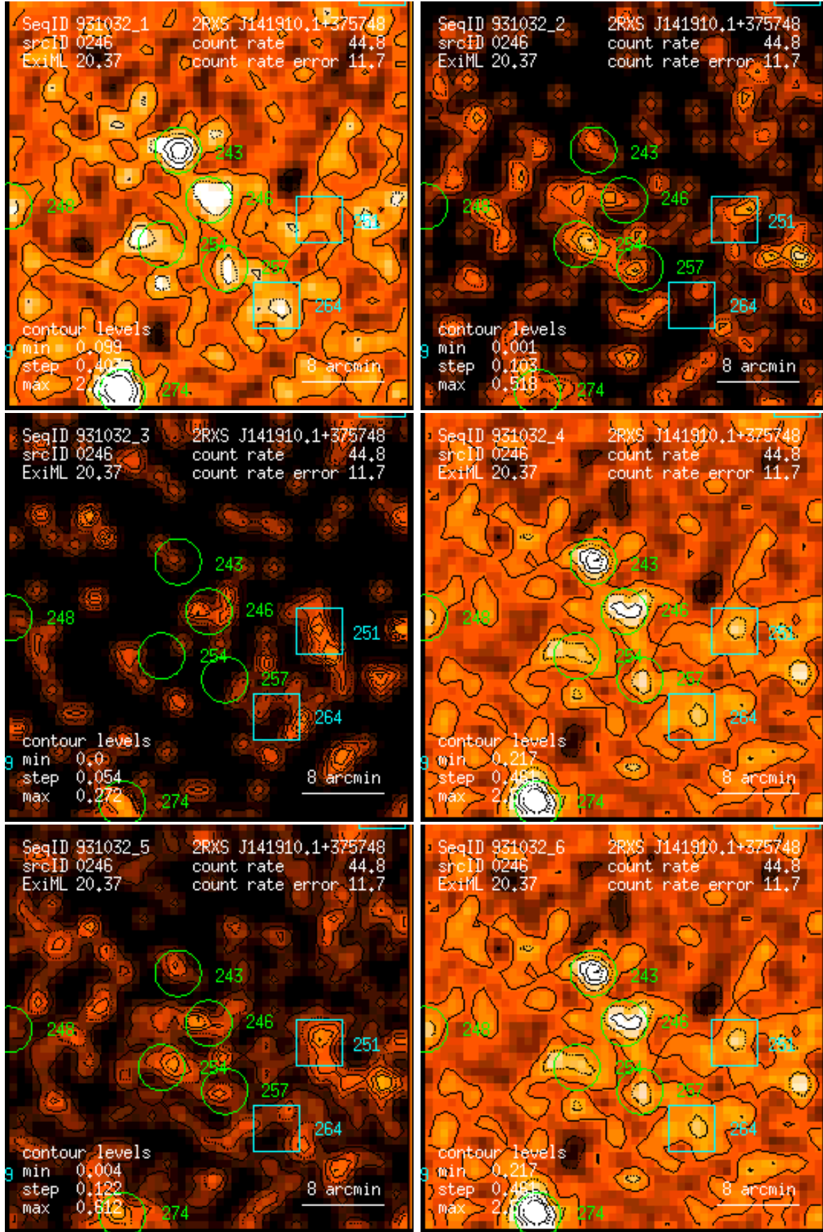
Figure 246: RASS 931032: detection 0246: band rate images, Gaussian filter: (1) PSPC channels 11 – 41, (2) 52 – 90, (3) 91 – 201, (4) 11 – 235, (5) 52 – 201, (6) 11 – 201. Broad band rates in counts/ks. Band rate contour levels in counts/ks/arcmin 2 .
