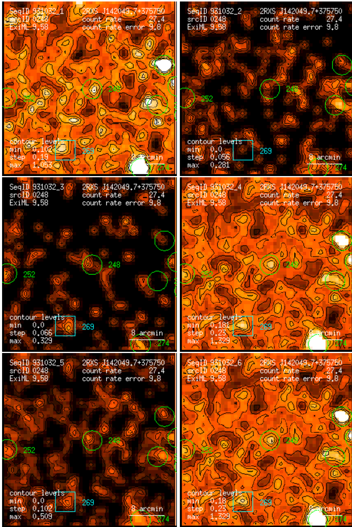
Figure 248: RASS 931032: detection 0248: band rate images, Gaussian filter: (1) PSPC channels 11 – 41, (2) 52 – 90, (3) 91 – 201, (4) 11 – 235, (5) 52 – 201, (6) 11 – 201. Broad band rates in counts/ks. Band rate contour levels in counts/ks/arcmin 2 .
