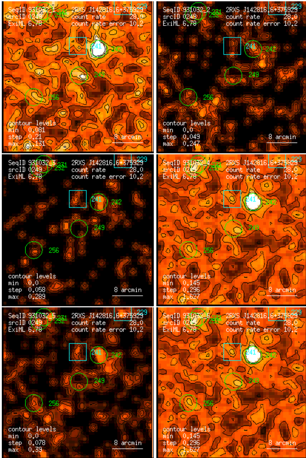
Figure 249: RASS 931032: detection 0249: band rate images, Gaussian filter: (1) PSPC channels 11 – 41, (2) 52 – 90, (3) 91 – 201, (4) 11 – 235, (5) 52 – 201, (6) 11 – 201. Broad band rates in counts/ks. Band rate contour levels in counts/ks/arcmin 2 .
