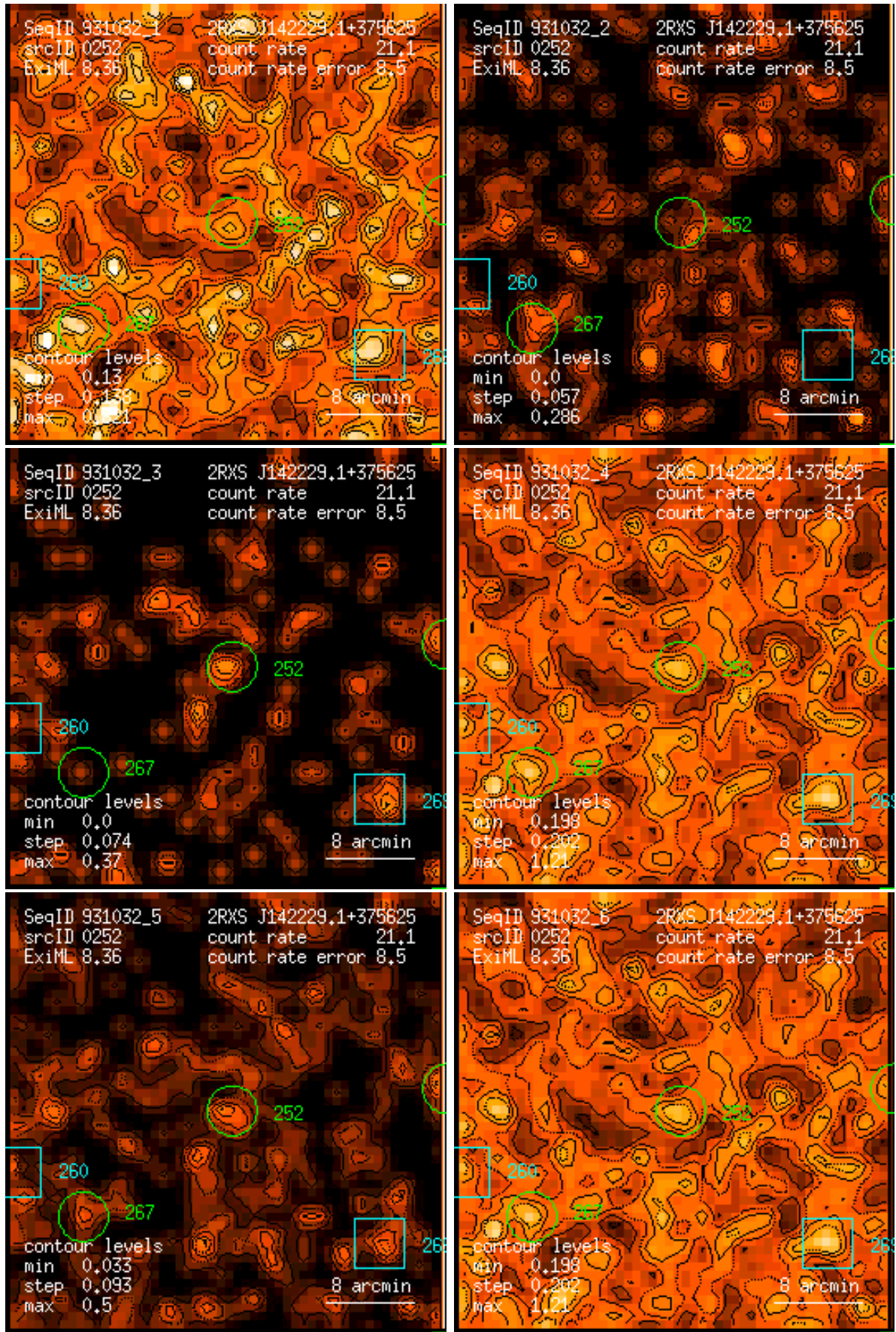
Figure 252: RASS 931032: detection 0252: band rate images, Gaussian filter: (1) PSPC channels 11 – 41, (2) 52 – 90, (3) 91 – 201, (4) 11 – 235, (5) 52 – 201, (6) 11 – 201. Broad band rates in counts/ks. Band rate contour levels in counts/ks/arcmin 2 .
