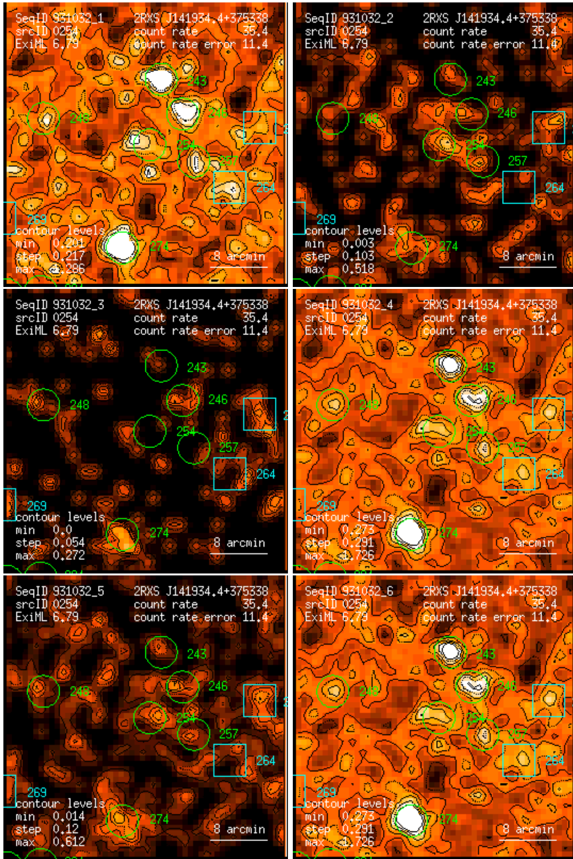
Figure 254: RASS 931032: detection 0254: band rate images, Gaussian filter: (1) PSPC channels 11 – 41, (2) 52 – 90, (3) 91 – 201, (4) 11 – 235, (5) 52 – 201, (6) 11 – 201. Broad band rates in counts/ks. Band rate contour levels in counts/ks/arcmin 2 .
