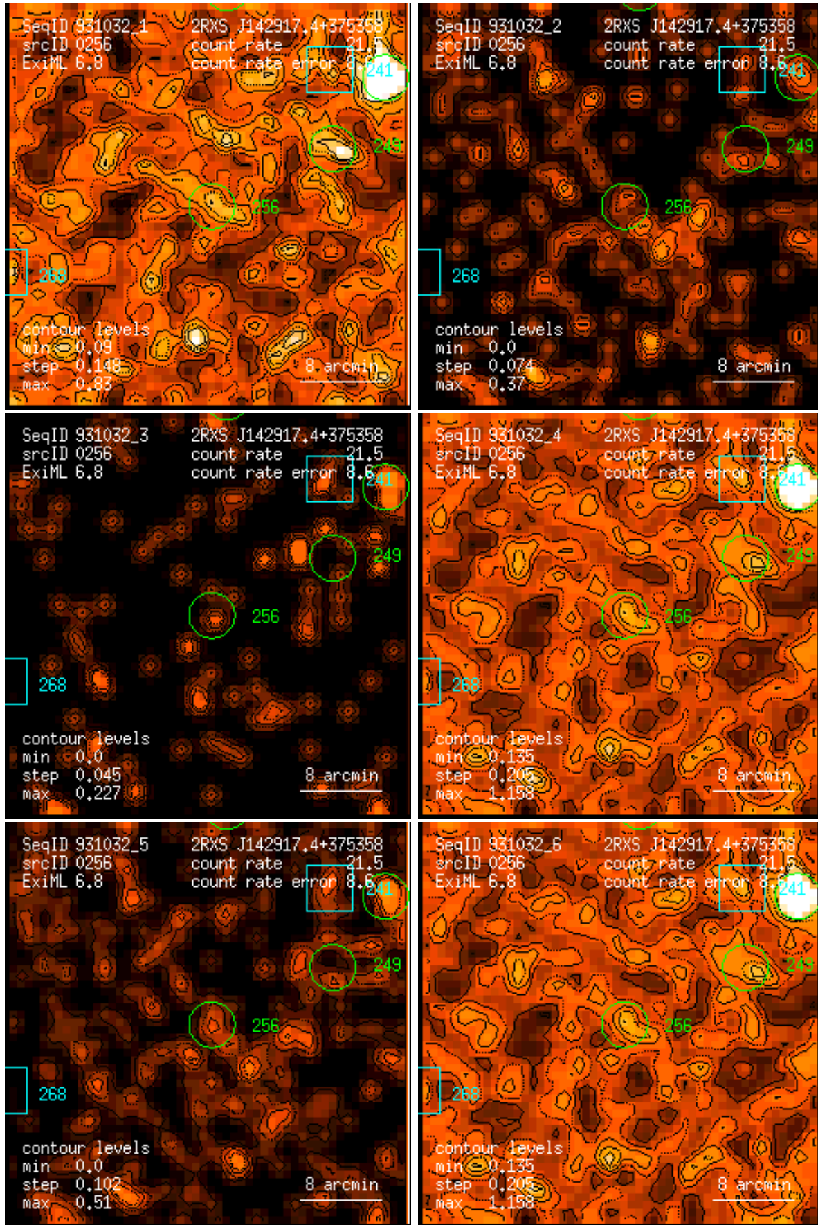
Figure 256: RASS 931032: detection 0256: band rate images, Gaussian filter: (1) PSPC channels 11 – 41, (2) 52 – 90, (3) 91 – 201, (4) 11 – 235, (5) 52 – 201, (6) 11 – 201. Broad band rates in counts/ks. Band rate contour levels in counts/ks/arcmin 2 .
