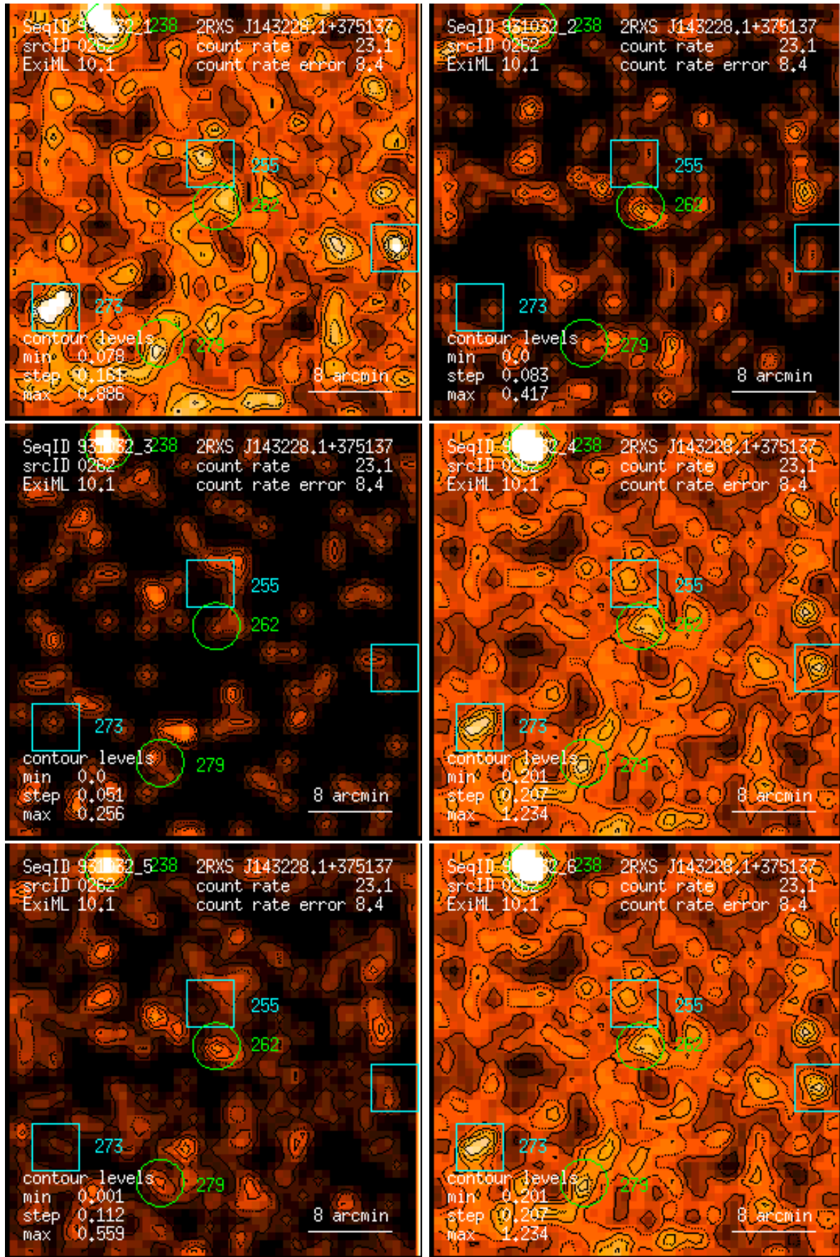
Figure 262: RASS 931032: detection 0262: band rate images, Gaussian filter: (1) PSPC channels 11 – 41, (2) 52 – 90, (3) 91 – 201, (4) 11 – 235, (5) 52 – 201, (6) 11 – 201. Broad band rates in counts/ks. Band rate contour levels in counts/ks/arcmin 2 .
