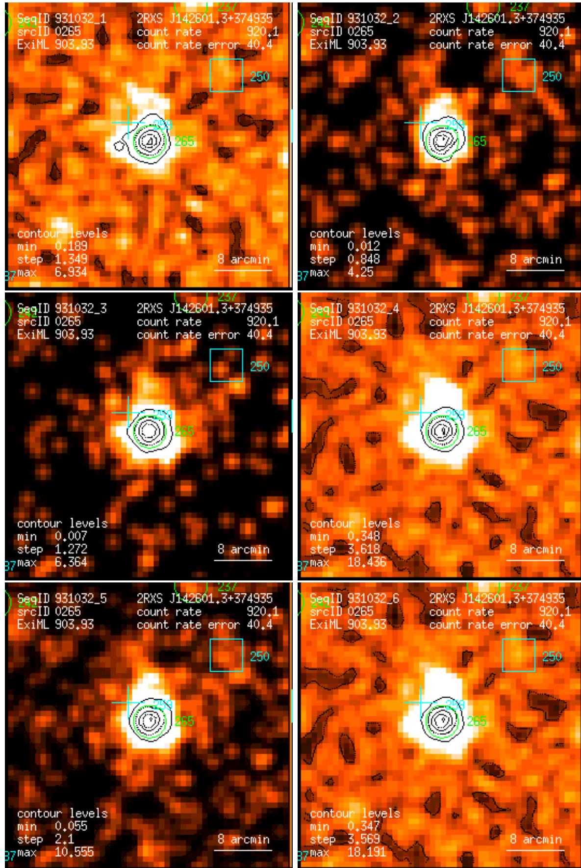
Figure 265: RASS 931032: detection 0265: band rate images, Gaussian filter: (1) PSPC channels 11 – 41, (2) 52 – 90, (3) 91 – 201, (4) 11 – 235, (5) 52 – 201, (6) 11 – 201. Broad band rates in counts/ks. Band rate contour levels in counts/ks/arcmin 2 .
