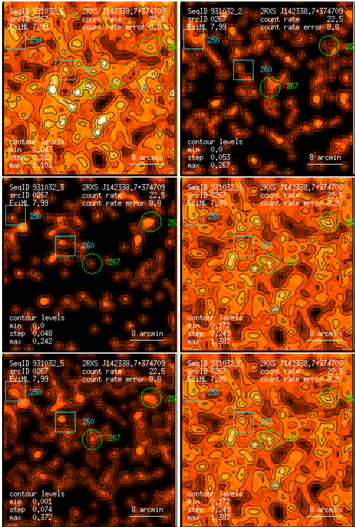
Figure 267: RASS 931032: detection 0267: band rate images, Gaussian filter: (1) PSPC channels 11 – 41, (2) 52 – 90, (3) 91 – 201, (4) 11 – 235, (5) 52 – 201, (6) 11 – 201. Broad band rates in counts/ks. Band rate contour levels in counts/ks/arcmin 2 .
