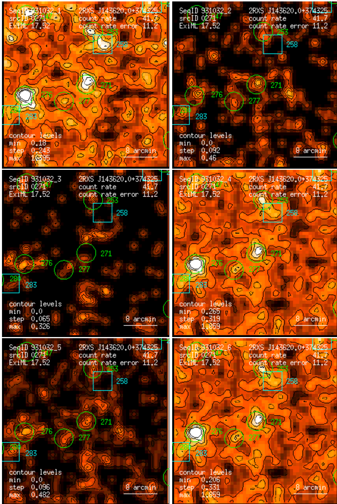
Figure 271: RASS 931032: detection 0271: band rate images, Gaussian filter: (1) PSPC channels 11 – 41, (2) 52 – 90, (3) 91 – 201, (4) 11 – 235, (5) 52 – 201, (6) 11 – 201. Broad band rates in counts/ks. Band rate contour levels in counts/ks/arcmin 2 .
