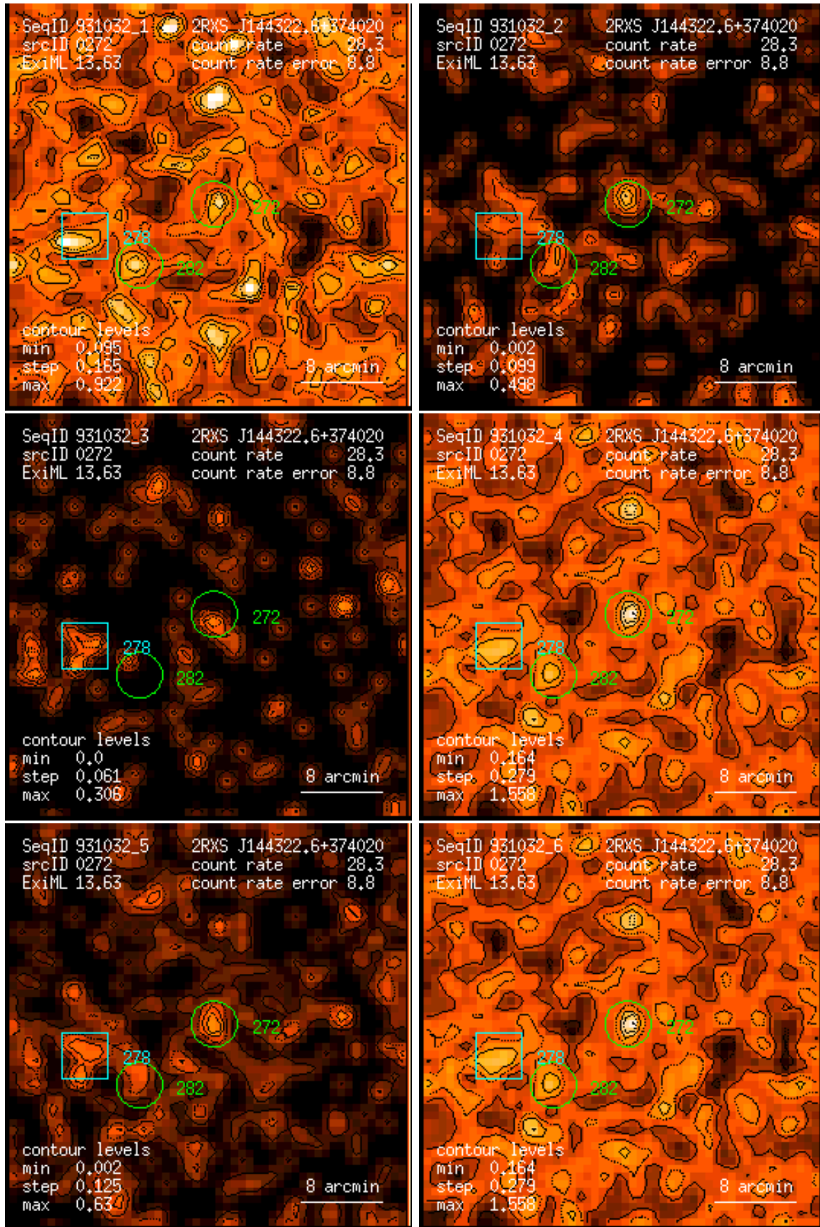
Figure 272: RASS 931032: detection 0272: band rate images, Gaussian filter: (1) PSPC channels 11 – 41, (2) 52 – 90, (3) 91 – 201, (4) 11 – 235, (5) 52 – 201, (6) 11 – 201. Broad band rates in counts/ks. Band rate contour levels in counts/ks/arcmin 2 .
