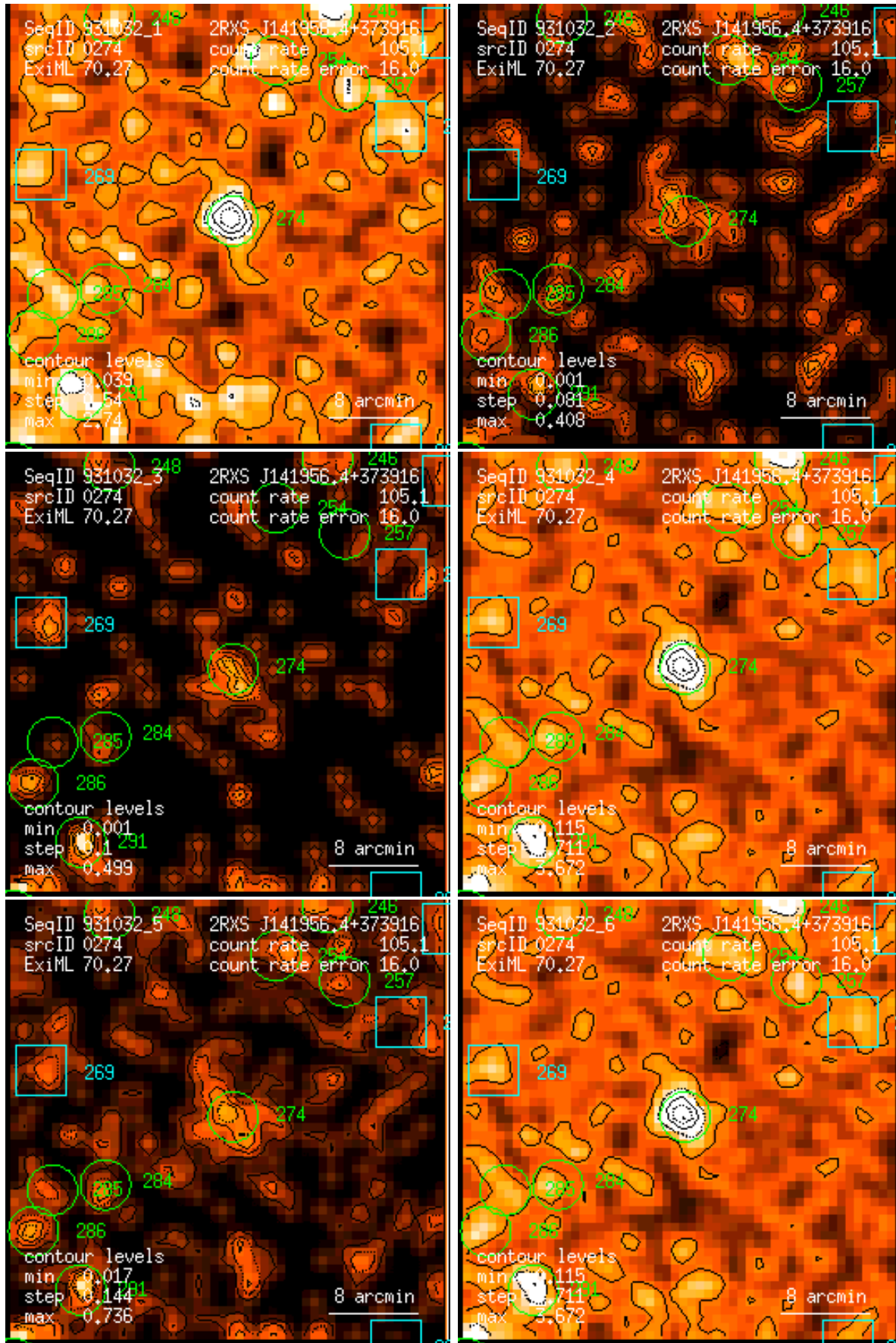
Figure 274: RASS 931032: detection 0274: band rate images, Gaussian filter: (1) PSPC channels 11 – 41, (2) 52 – 90, (3) 91 – 201, (4) 11 – 235, (5) 52 – 201, (6) 11 – 201. Broad band rates in counts/ks. Band rate contour levels in counts/ks/arcmin 2 .
