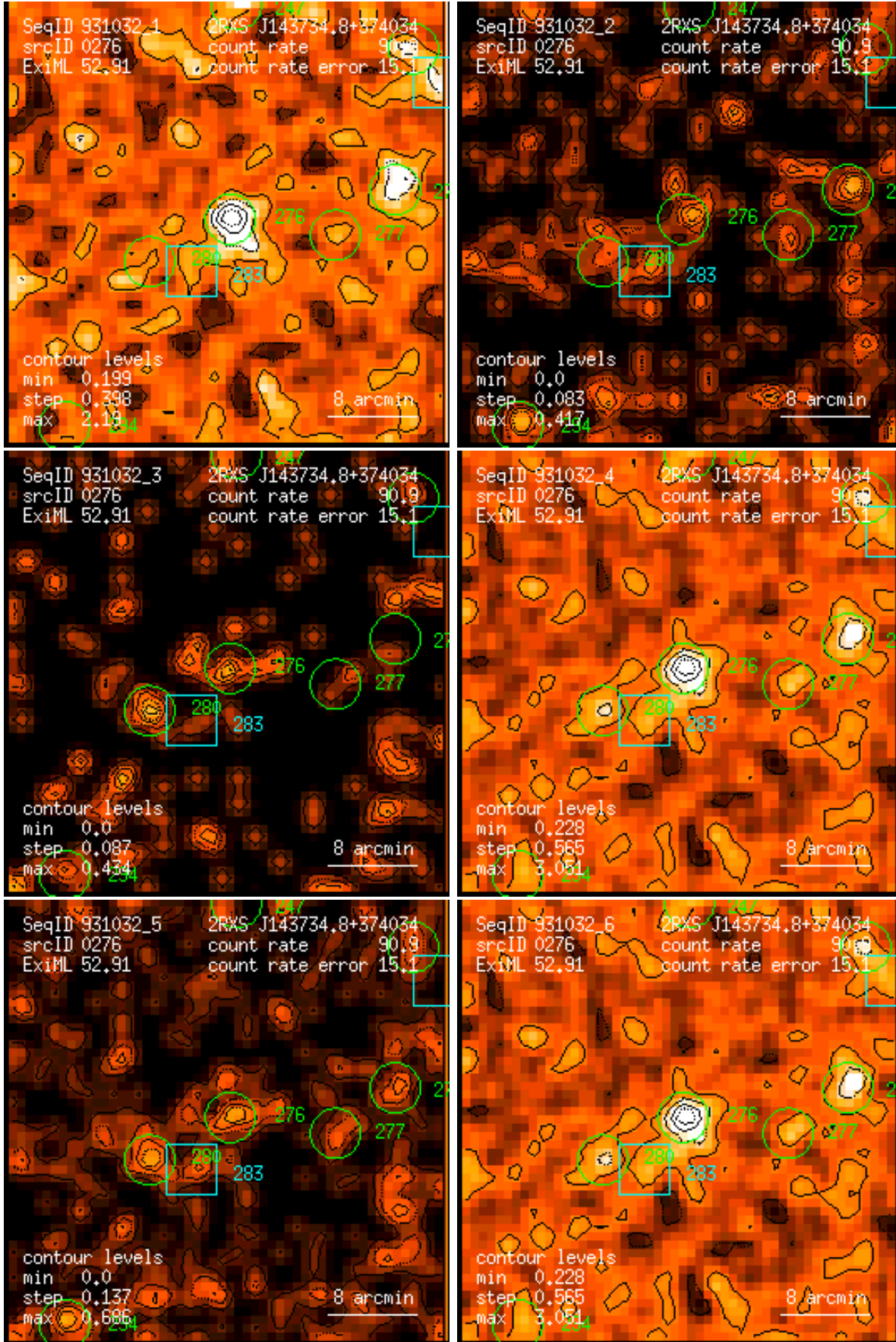
Figure 276: RASS 931032: detection 0276: band rate images, Gaussian filter: (1) PSPC channels 11 – 41, (2) 52 – 90, (3) 91 – 201, (4) 11 – 235, (5) 52 – 201, (6) 11 – 201. Broad band rates in counts/ks. Band rate contour levels in counts/ks/arcmin 2 .
