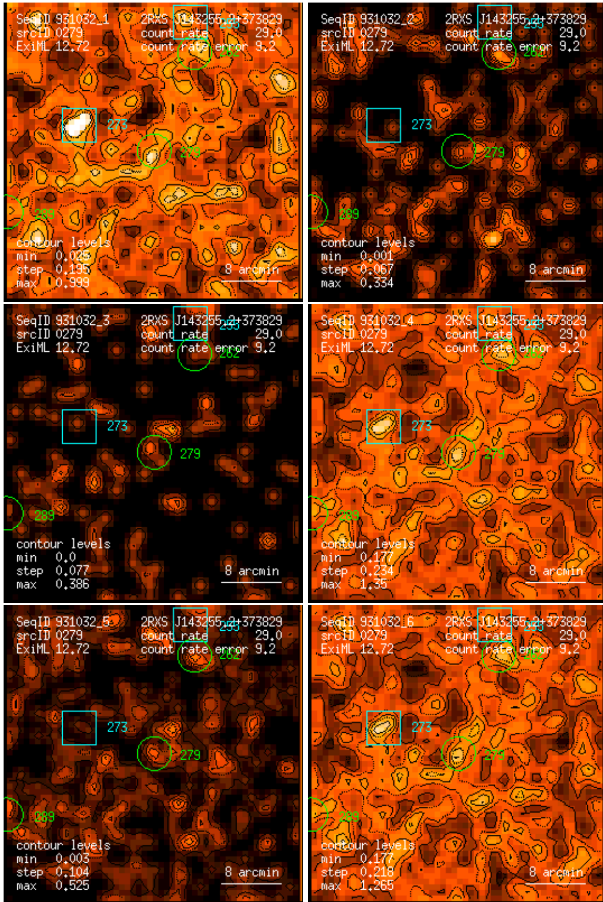
Figure 279: RASS 931032: detection 0279: band rate images, Gaussian filter: (1) PSPC channels 11 – 41, (2) 52 – 90, (3) 91 – 201, (4) 11 – 235, (5) 52 – 201, (6) 11 – 201. Broad band rates in counts/ks. Band rate contour levels in counts/ks/arcmin 2 .
